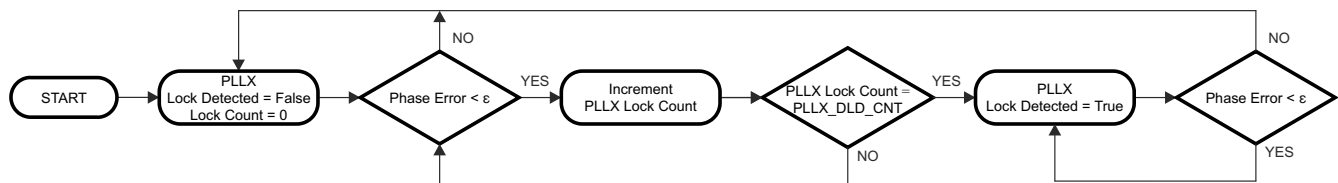
図 8-8. Digital Lock Detect Flowchart
