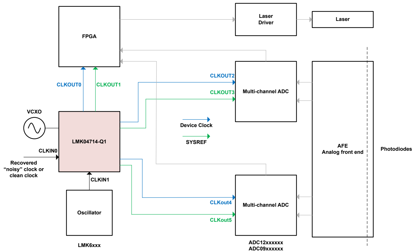
図 9-15. Typical LIDAR Automotive Application
