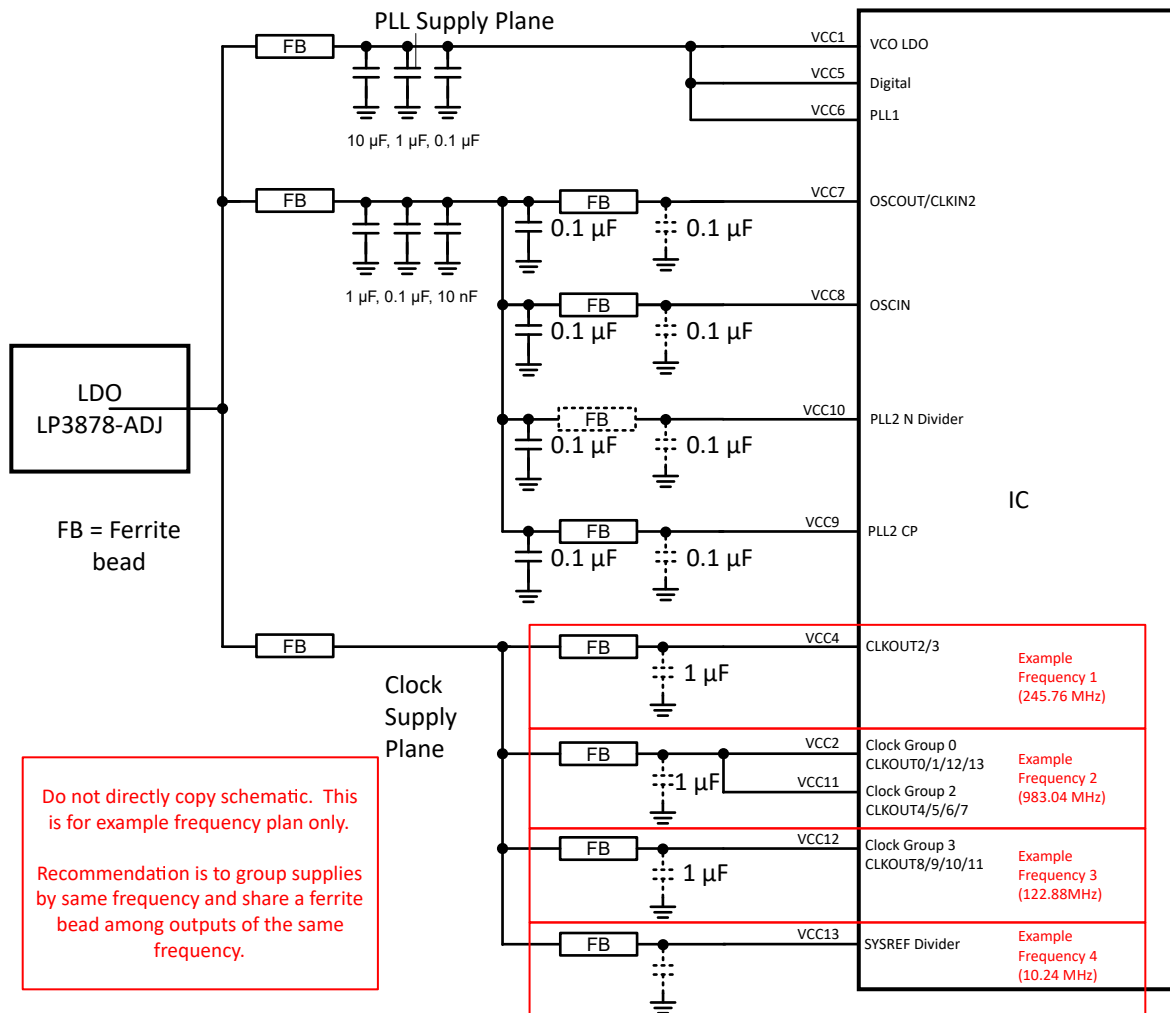
図 9-17. Example Application - Power System Schematic
