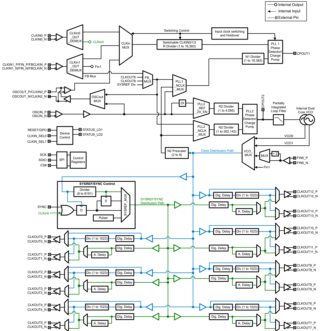
図 8-1. High Level Block Diagram
