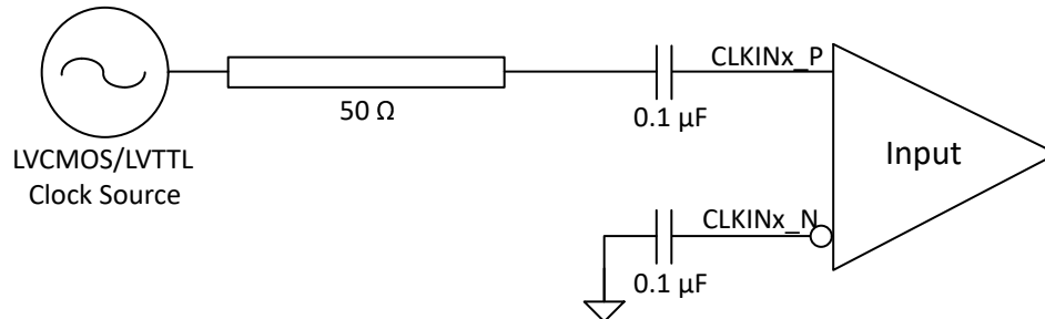
図 9-5. DC-Coupled LVCMOS/LVTTL Reference Clock
