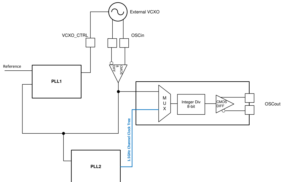
Figure 35. OSCout Block
