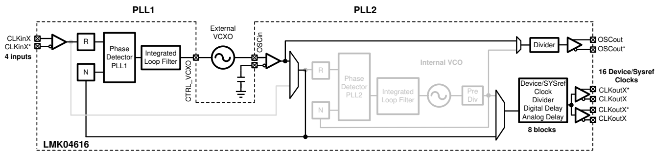
Figure 53. Simplified Functional Block Diagram for PLL1 Only or PLL2 Bypass Mode
