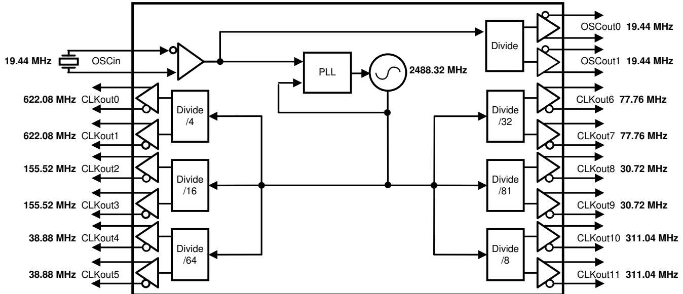
FIG 7-4. SONET/SDH Reference Clocks
