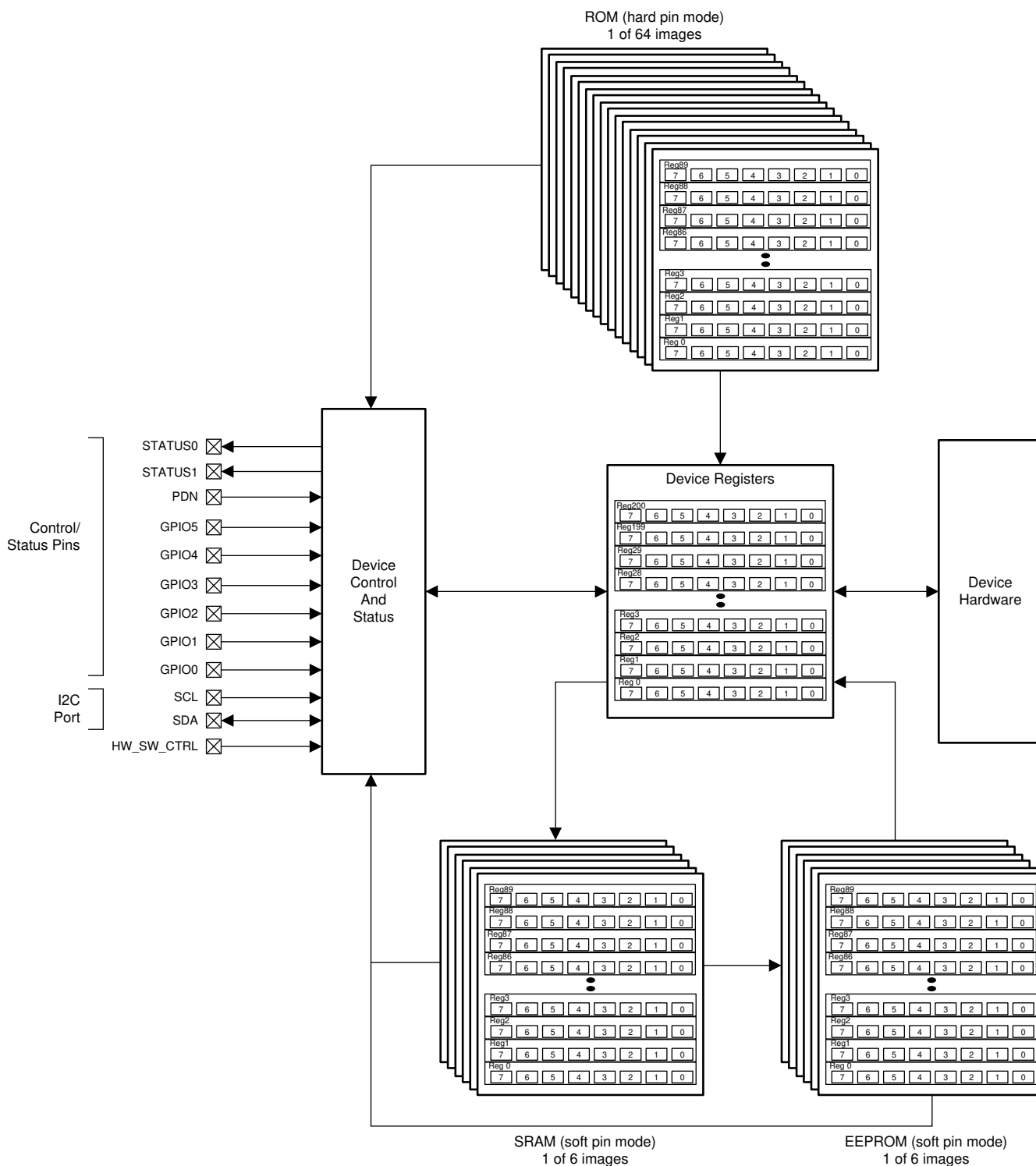
8-30. LMK03328 Interface and Control Block
