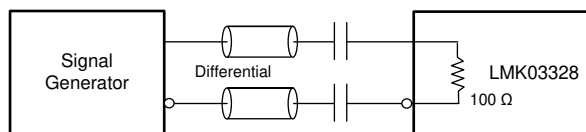
7-12. Differential Input AC Configuration During Device Test
