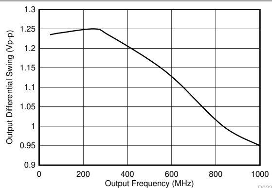
図 6-20. AC-CML Differential Output Swing vs. Frequency
