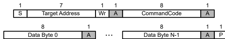
Figure 8-34. Block Register Write Programming Sequence
