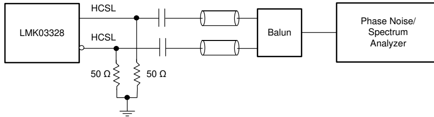
図 7-6. HCSL Output AC Configuration During Device Test
