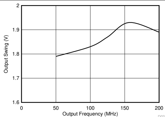
図 6-22. 1.8-V LVCMOS (on OUT[7:0]) Output Swing vs. Frequency
