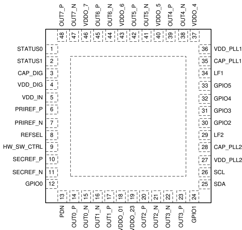
図 5-1. RHS Package 48-Pin WQFN Top View
