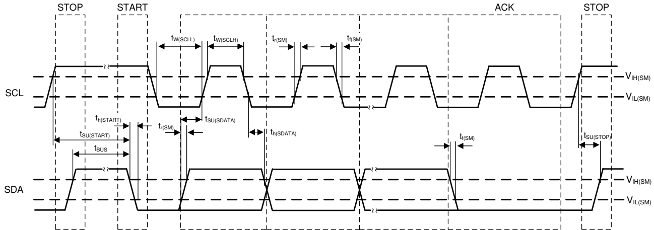
図 8-31. I 2 C Timing Diagram
