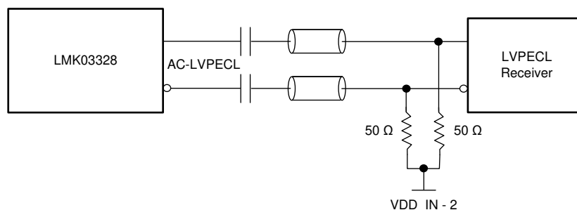
図 8-25. Interfacing the LMK03328 AC-LVPECL Output With LVPECL Receiver
