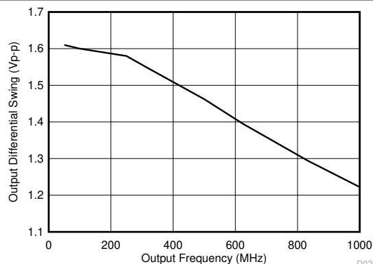
図 6-18. AC-LVPECL Differential Output Swing vs. Frequency
