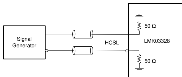
図 7-11. HCSL Input DC Configuration During Device Test
