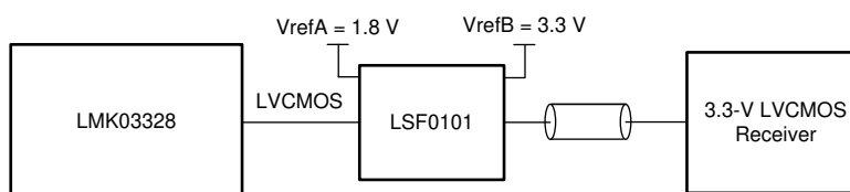
図 8-24. Interfacing the LMK03328 1.8-V LVCMOS Output With 3.3-V LVCMOS Receiver
