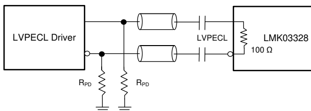
8-12. AC-Coupling LMK03328 Inputs With LVPECL Signal
