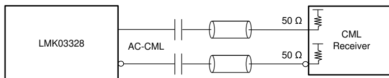
図 8-27. Interfacing the LMK03328 AC-CML Output With CML Receiver
