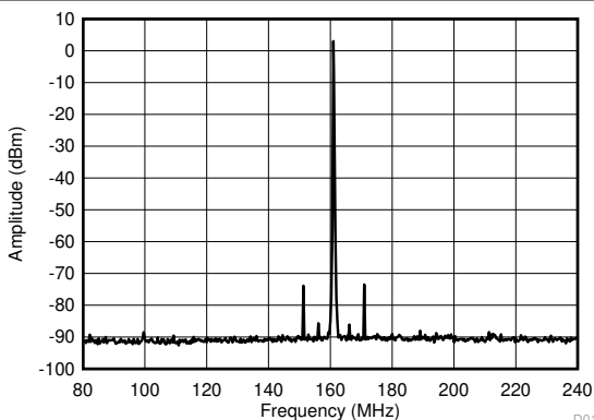
図 6-17. 161.1328125 ± 80.56640625-MHz HCSL Output Spectrum With PLL Bandwidth at 400 kHz, Fractional N PLL, 50-MHz Crystal Input, 5.15625-GHz VCO Frequency, Post Divider = 8, Output Divider = 4
