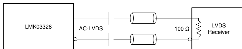
図 8-26. Interfacing the LMK03328 AC-LVDS Output With LVDS Receiver
