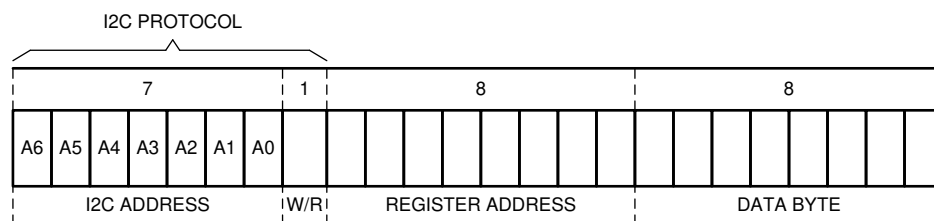
図 8-32. I 2 C Register Structure
