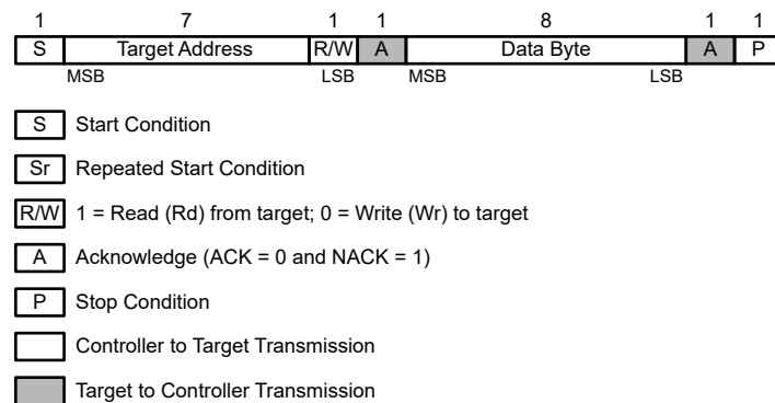
図 8-33. Generic Programming Sequence
