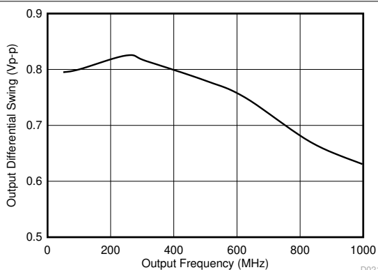
図 6-19. AC-LVDS Differential Output Swing vs. Frequency
