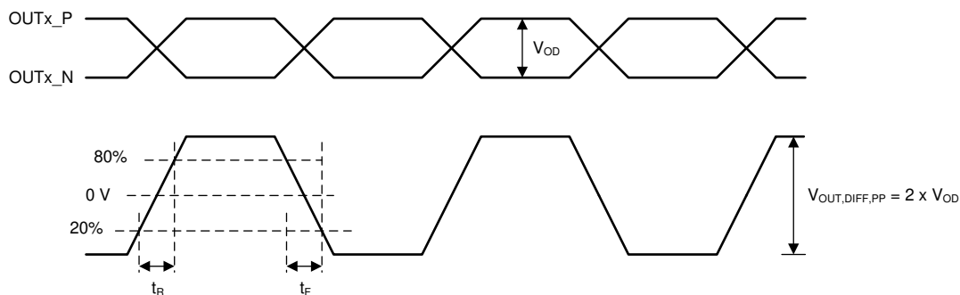
7-15. Differential Output Voltage and Rise/Fall Time
