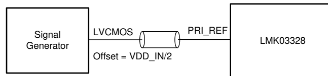
図 7-7. LVCMOS Primary Input DC Configuration During Device Test
