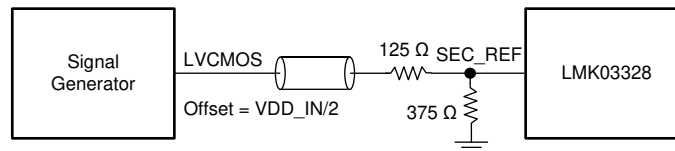
図 7-8. LVCMOS Secondary Input DC Configuration During Device Test
