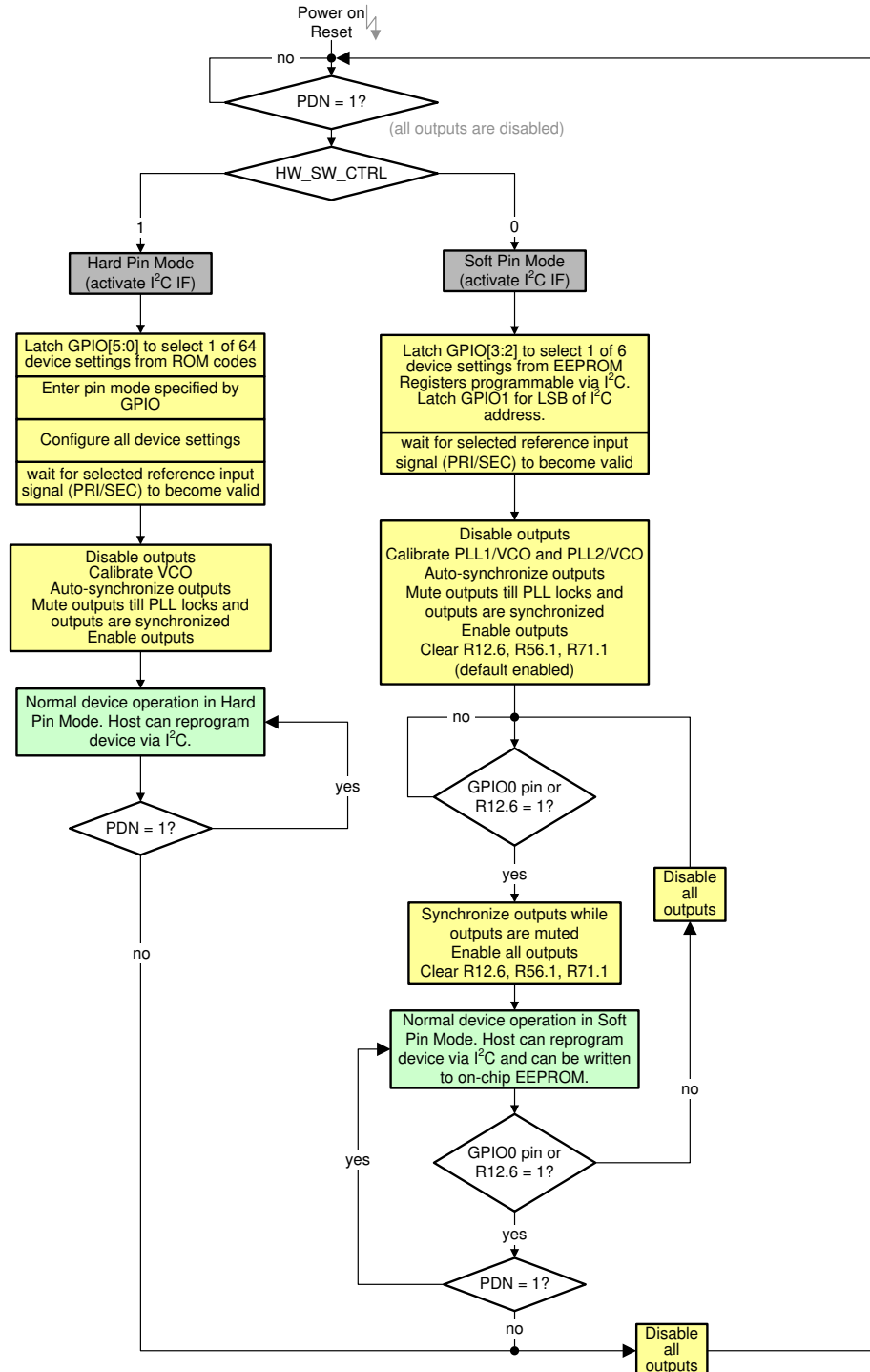
図 10-9. Flow Chart for Device Power Up and Configuration
