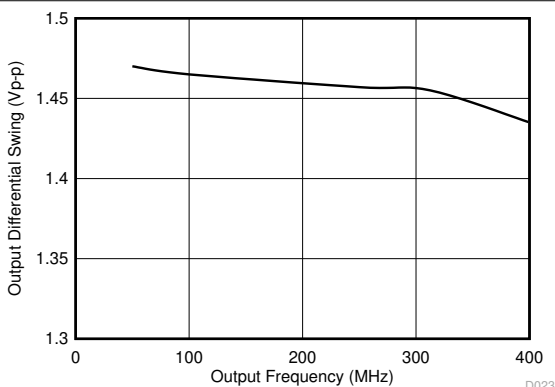
図 6-21. HCSL Differential Output Swing vs. Frequency
