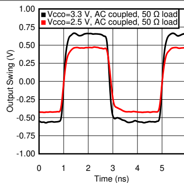
6-2. LVCMOS Output Swing at 250 MHz
