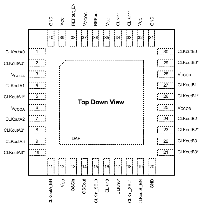
图 5-1. RTA Package 40-Pin WQFN Top View
