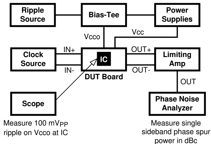
FIG 9-1. PSRR Test Setup
