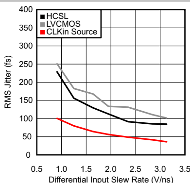
6-5. RMS Jitter vs CLKIn Slew Rate at 100 MHz
