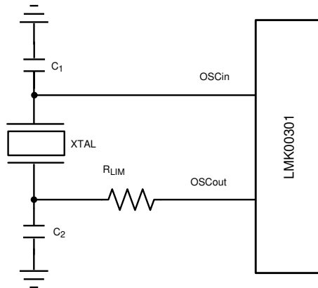
Figure 9-5. Crystal Interface
