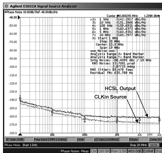
6-11. HCSL Phase Noise at 100 MHz
