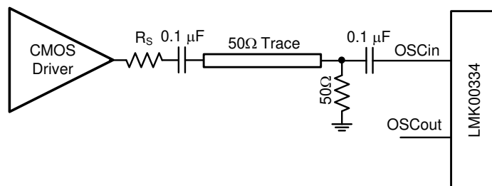
Figure 9-4. Driving OSCin With a Single-Ended Input
