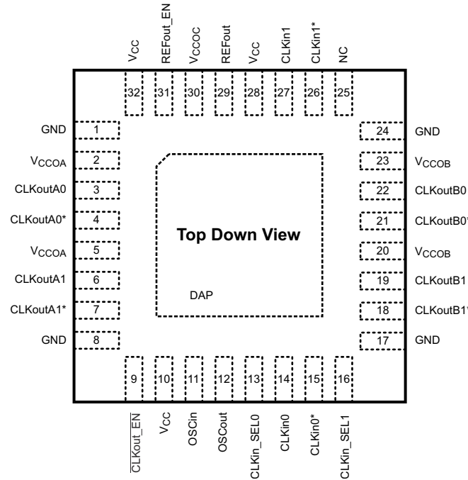
图 5-1. RTV Package 32-Pin WQFN Top View
