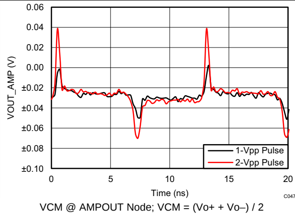
FIG 52. SE-DE Output Common Mode Pulse Response
