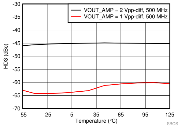
FIG 46. SE-DE 3rd Order Harmonic Distortion vs Temperature
