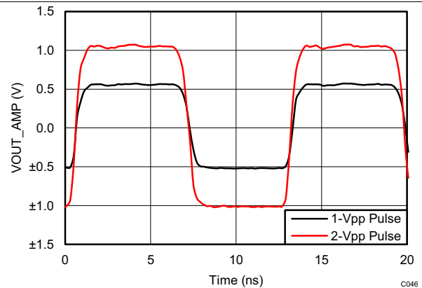
FIG 51. SE-DE Output Signal Pulse Response
