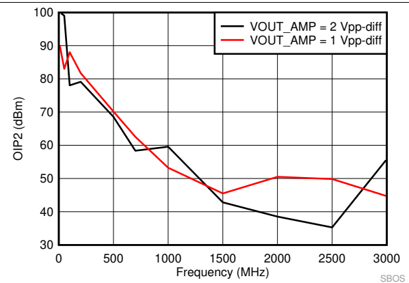
FIG 47. SE-DE 2nd Order Intermodulation Distortion vs Frequency
