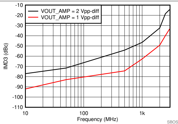
FIG 48. SE-DE 3rd Order Intermodulation Distortion vs Frequency
