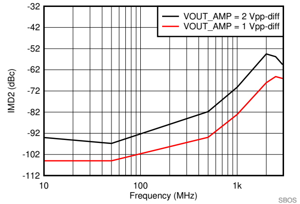
FIG 47. SE-DE 2nd Order Intermodulation Distortion vs Frequency
