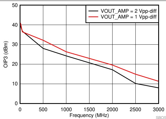
FIG 48. SE-DE 3rd Order Intermodulation Distortion vs Frequency
