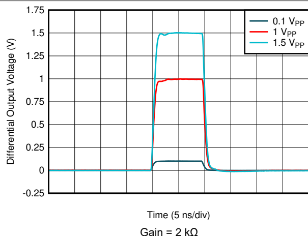
6-19. Pulse Response vs Output Swing
