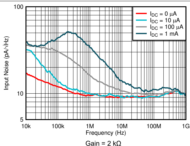
6-15. Input Noise Density vs Ambient-Light DC Current
