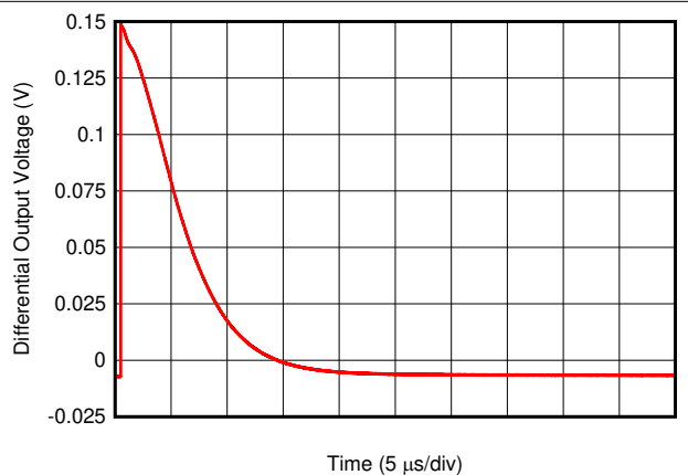
6-25. Turn-Off Time
