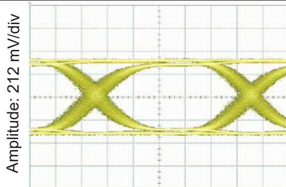
Time: 50 ps/div Figure 5. 100-M B1694A PRBS10 2.97 Gbps
