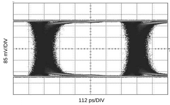
FIG 21. 1.485 Gbps, CC = 280 m Belden 1694A
