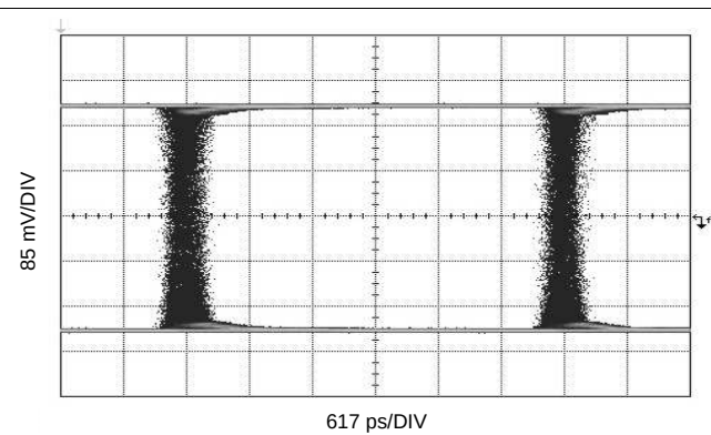
FIG 22. 270 Mbps, CC = 400 m Belden 1694A
