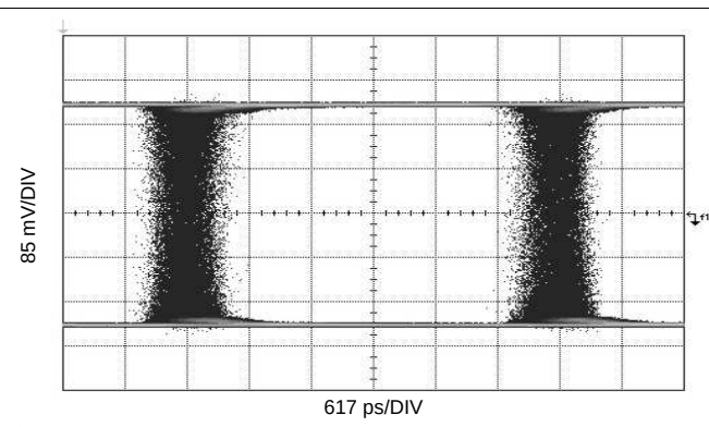
FIG 23. 270 Mbps, CC = 600 m Belden 1694A
