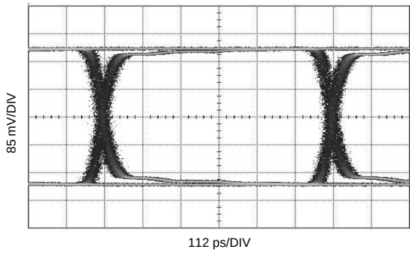
FIG 20. 1.485 Gbps, CC = 200 m Belden 1694A
