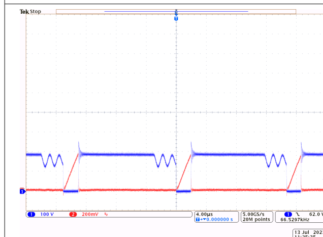
図 8-4. V_{IN} = 115VAC V_{OUT} = 5V I_{OUT} = 3A
