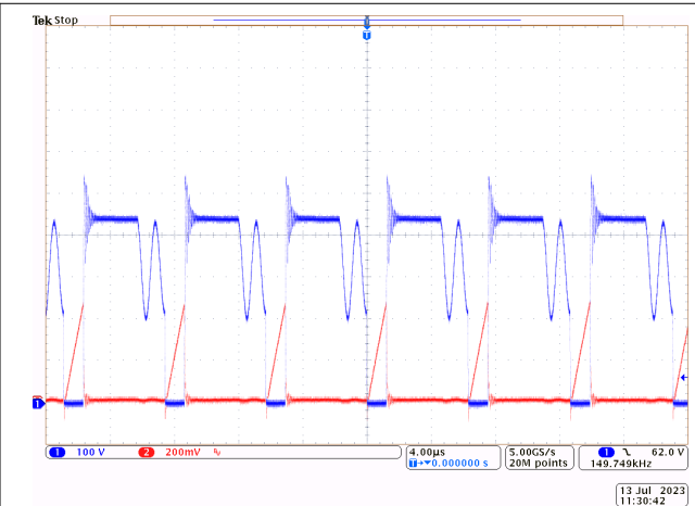
図 8-3. V_{IN} = 230VAC V_{OUT} = 20V I_{OUT} = 3.25A
