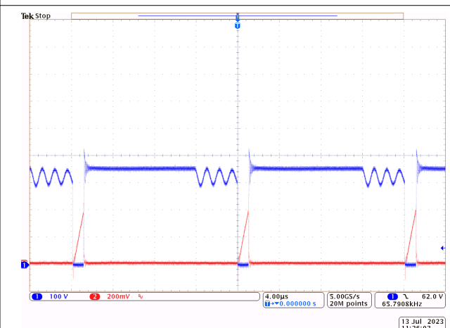
図 8-5. V_{IN} = 230VAC V_{OUT} = 5V I_{OUT} = 3A
