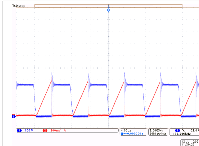
図 8-2. V_{IN} = 115VAC V_{OUT} = 20V I_{OUT} = 3.25A
