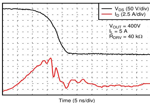
図 8-5. Turn-On Waveform in Application Example
