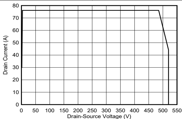
図 5-11. Repetitive Safe Operation Area
