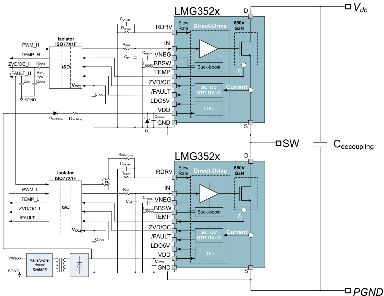
8-2. Typical Half-Bridge Application With Bootstrap
