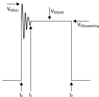
図 7-1. Drain-Source Voltage Switching Cycle
