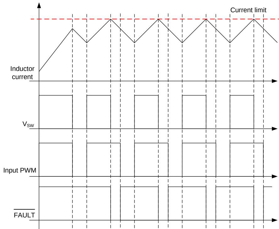
FIG 13. Cycle-by-cycle OCP Operation
