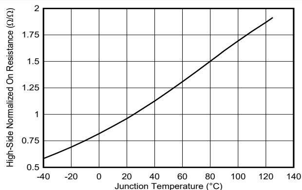
FIG 6-2. High-Side Normalized On-Resistance vs Junction Temperature
