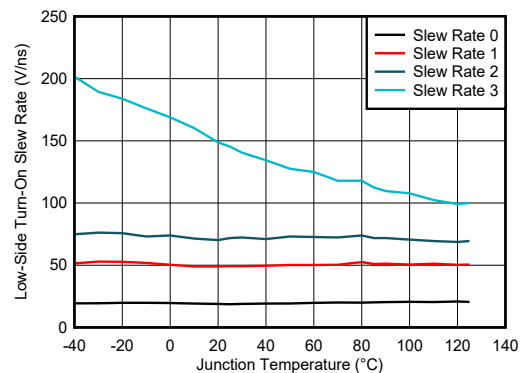
FIG 6-10. Low-Side Turn-On Slew Rate vs Junction Temperature
