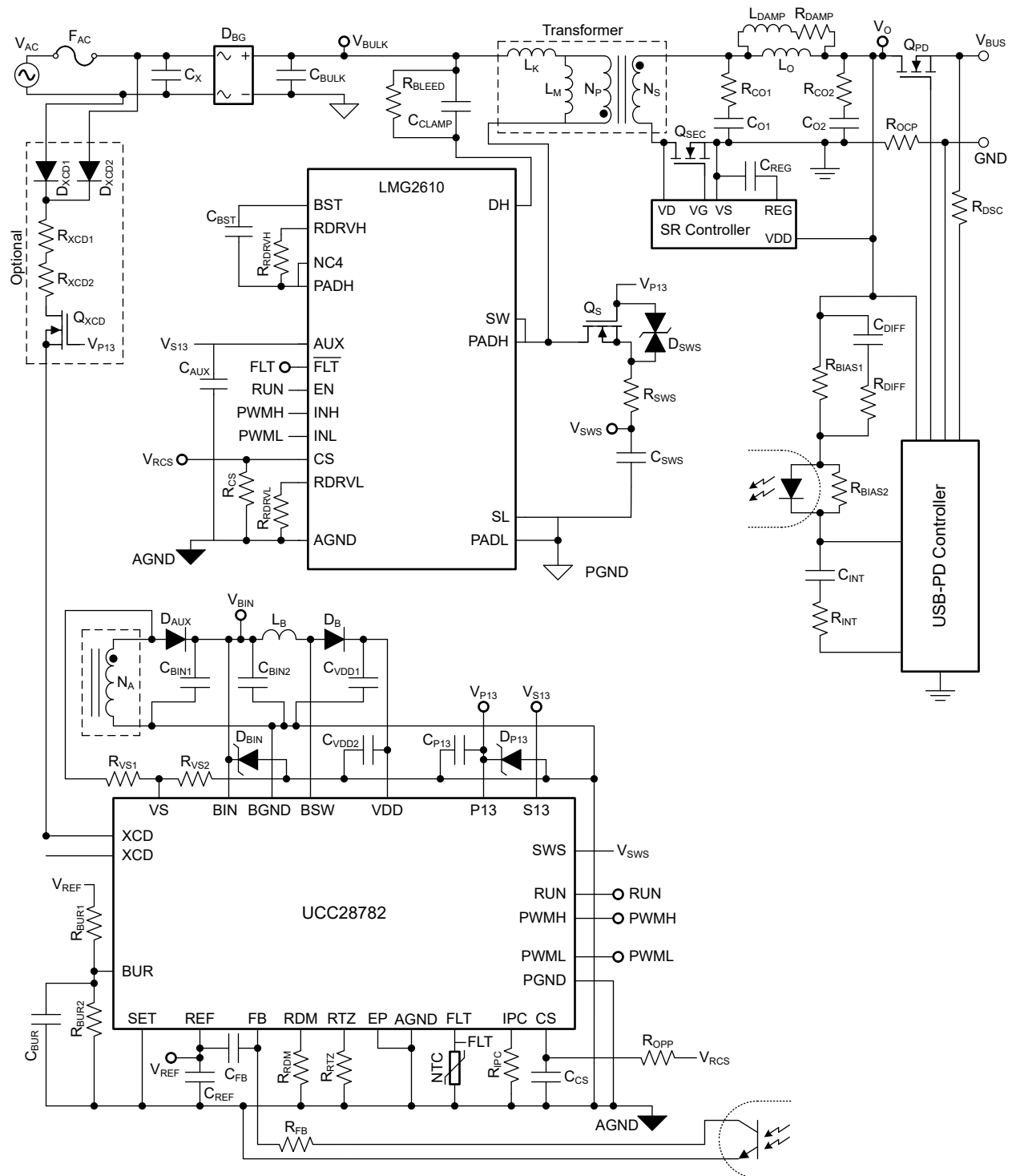
FIG 9-1. 65-W USB-PD Charger Application
