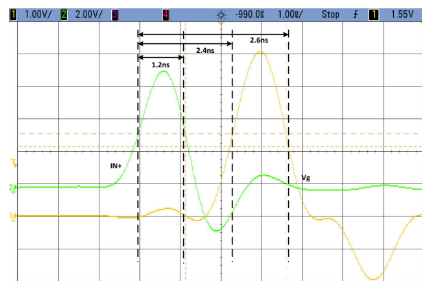
図 7-8. Input Pulse Width and Propagation Delays
