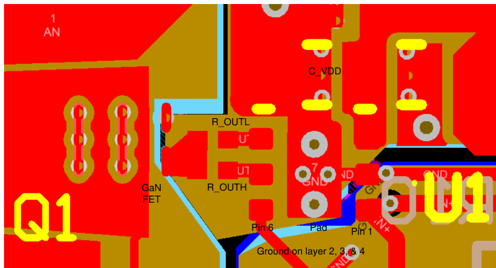
図 9-1. Typical LMG1025-Q1 Layout With Ball-Grid GaN FET
