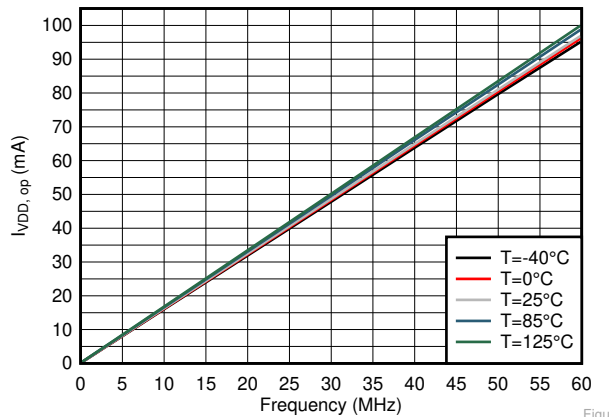
Figure 5-1. I_{VDD,op} with 2 \Omega in Series with 100pF Load
