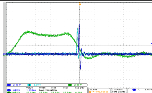
⊠ 12. 90 ns Pulse from Function Generator Yielding 1.5 ns Pulse On The Input (Cyan) And Gate (Blue) After Pulse Shortening
