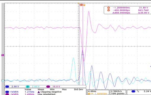
⊠ 13. 1.2 ns Gate Pulse Yielding 1.5 ns 30V Into 1 Ω Pulse (500MHz Scope)
