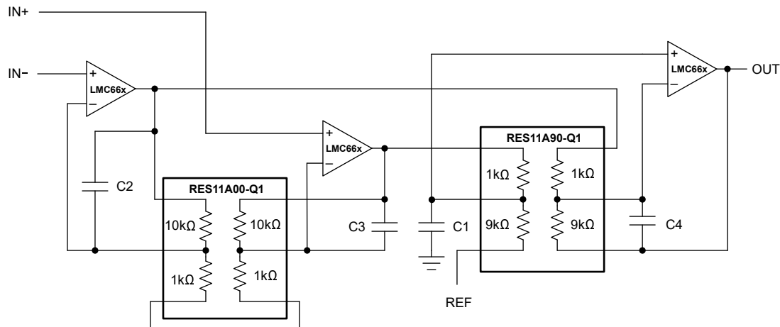
図 6-8. Improved Instrumentation Amplifier With the RES11A
