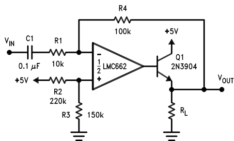
FIG 6-11. Power Amplifier
