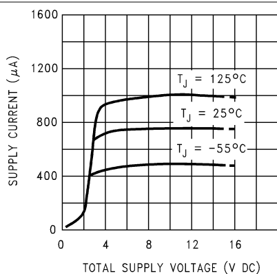
図 5-1. Supply Current vs Supply Voltage
