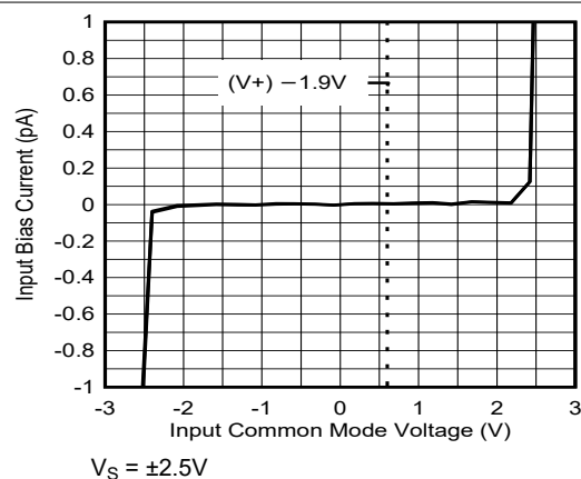
図 5-6. Input Bias Current vs Input Common-Mode Voltage
