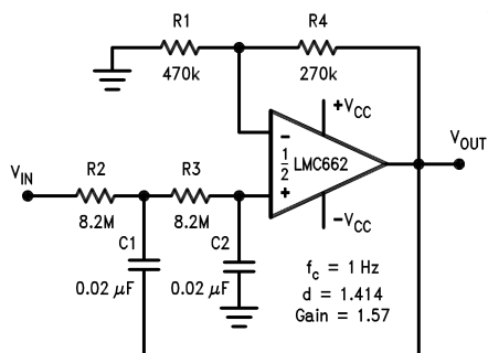
6-14. 1Hz Low Pass Filter (Maximally Flat, Dual Supply Only)
