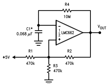
FIG 6-10. 1Hz Square-Wave Oscillator
