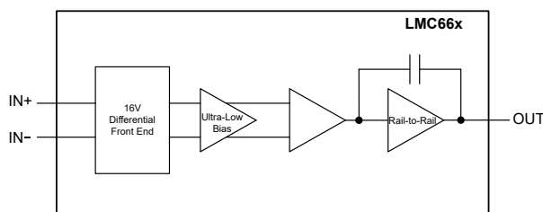
図 6-1. LMC66x Circuit Topology (Each Amplifier)
