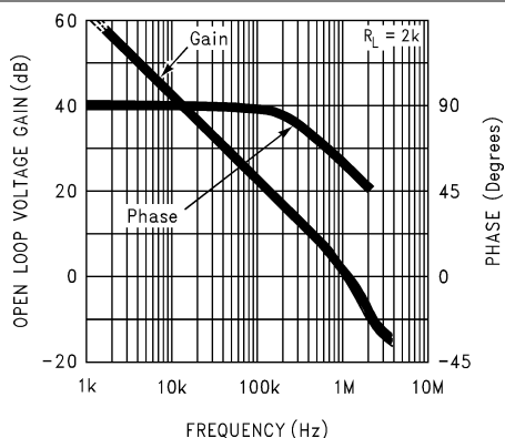
Figure 5-13. Gain and Phase Response vs Temperature
