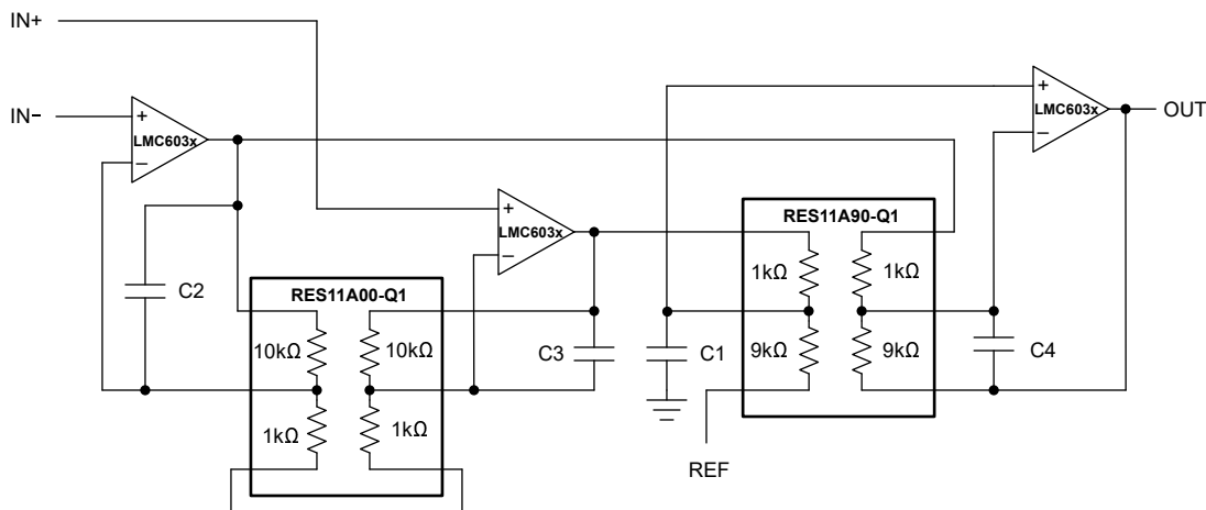
图 6-7. Improved Instrumentation Amplifier With RES11A
