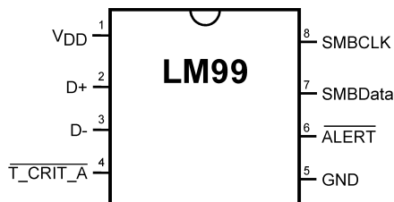
Figure 1. VSSOP-8 TOP VIEW
