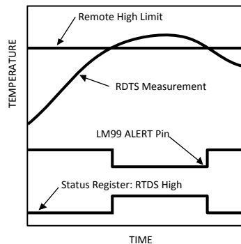
Figure 5. ALERT Comparator Temperature Response Diagram
