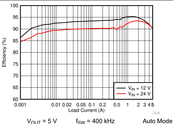
8-4. LM76005 Efficiency
