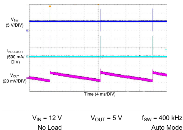
8-8. LM76005 Switching Waveform and Output Ripple
