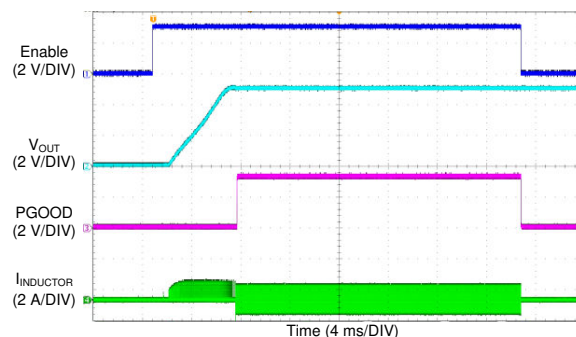
8-17. LM76005 Start-up Waveform
