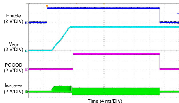
8-16. LM76005 Start-up Waveform
