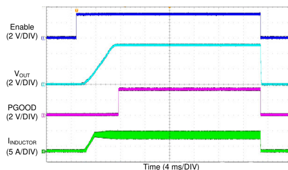
8-19. LM76005 Start-up Waveform
