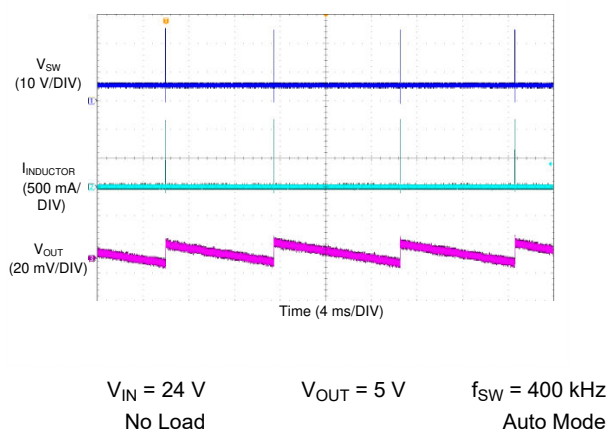
8-9. LM76005 Switching Waveform and Output Ripple
