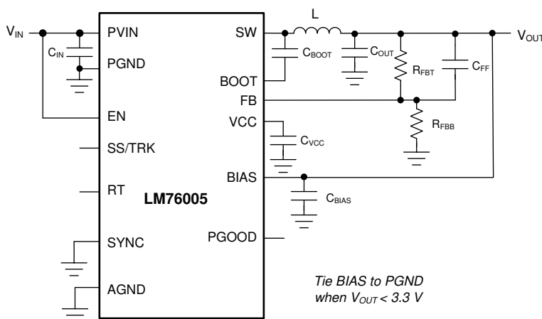
8-1. LM76005 Basic Schematic
