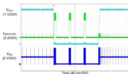
8-22. LM76005 Start-up With Pre-Biased Output
