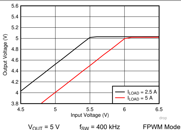
8-6. LM76005 Voltage Dropout
