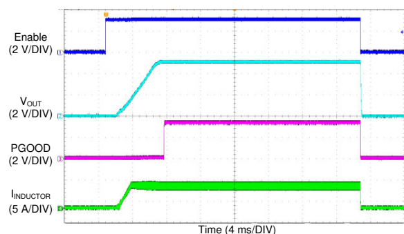
8-18. LM76005 Start-up Waveform
