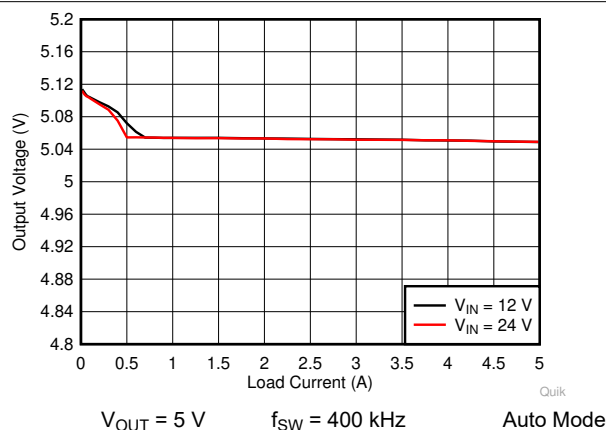
8-5. LM76005 Load and Line Regulation
