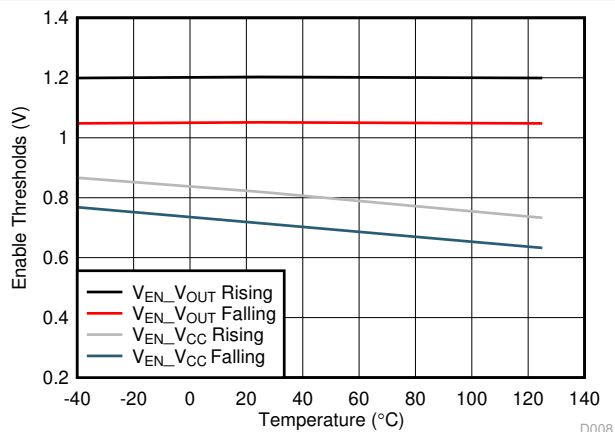
Figure 6-4. Enable Threshold
