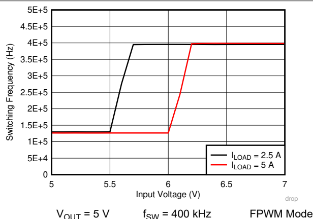
8-7. LM76005 Frequency Dropout
