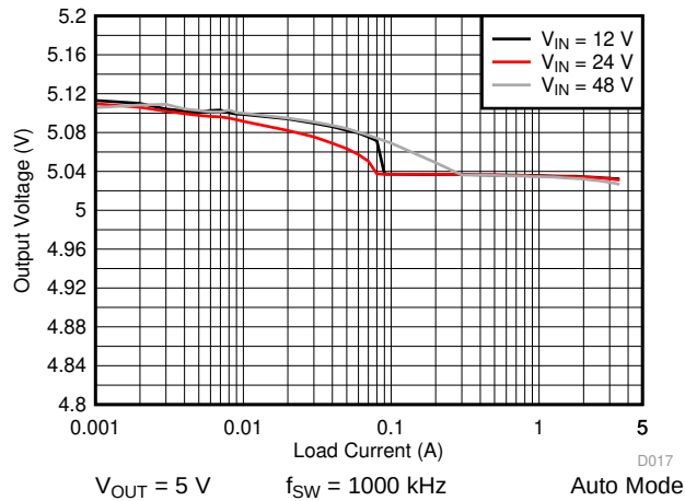
图 41. LM76003 Load and Line Regulation
