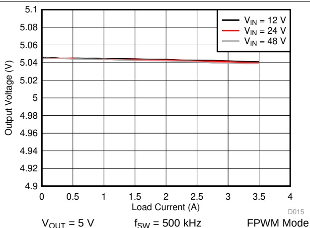
图 40. LM76003 Load and Line Regulation
