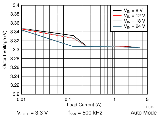
图 37. LM76003 Load and Line Regulation
