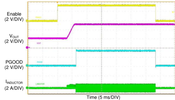
FIG 68. LM76002 Start-up Waveform
