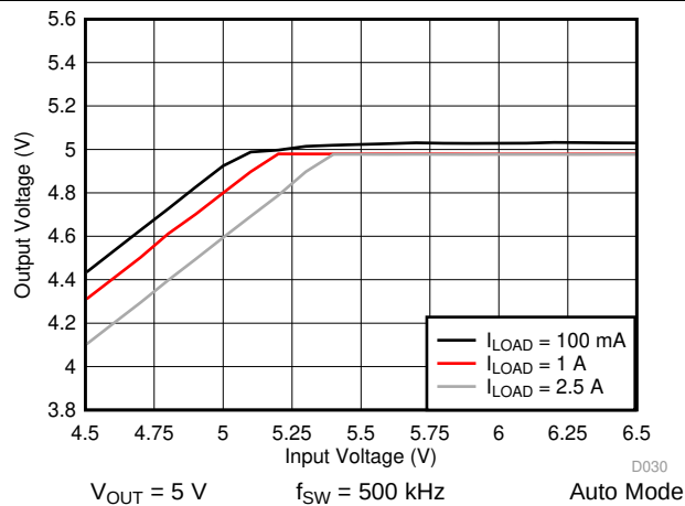
图 55. LM76002 Dropout Curve
