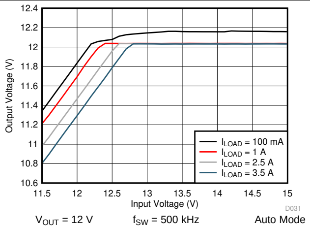
图 56. LM76003 Dropout Curve
