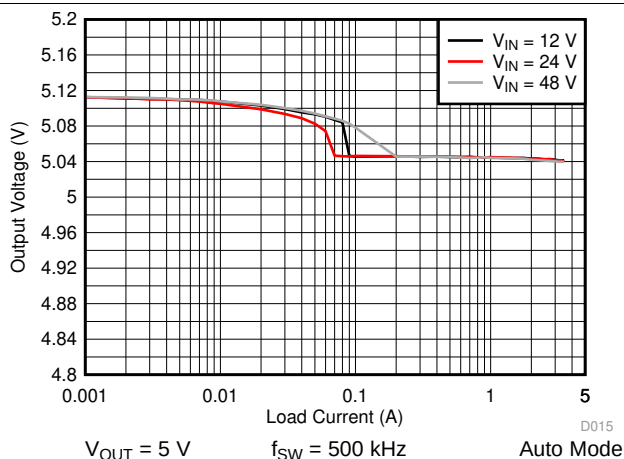
图 39. LM76003 Load and Line Regulation
