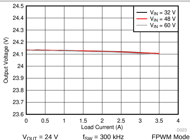
图 48. LM76003 Load and Line Regulation
