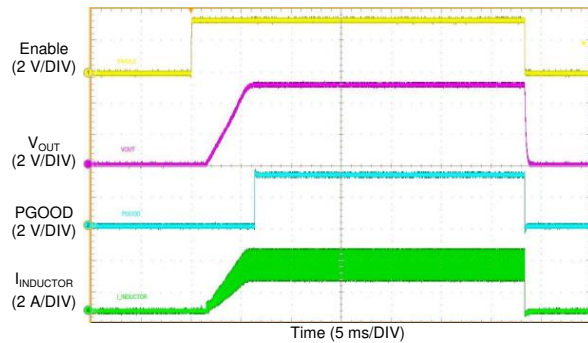
FIG 65. LM76003 Start-up Waveform
