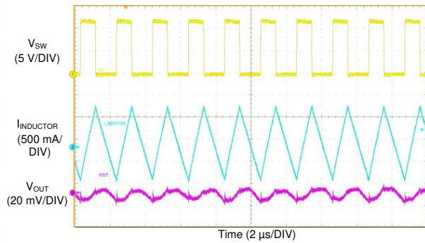
图 59. LM76003 Switching Waveform and Output Ripple
