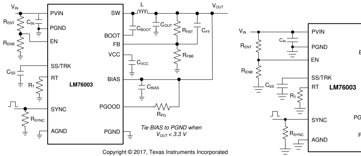
图 22. LM76002/LM76003 Comprehensive Schematic
