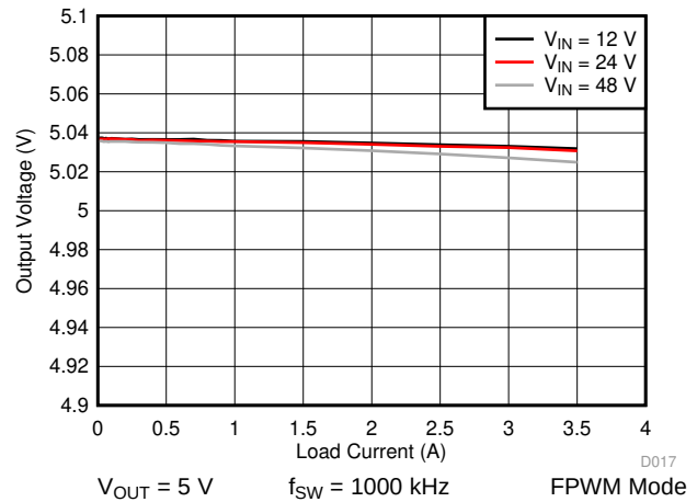
图 42. LM76003 Load and Line Regulation
