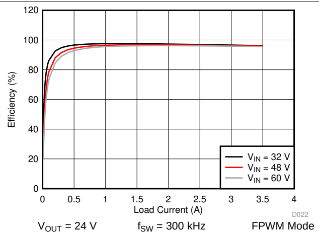
图 34. LM76003 Efficiency
