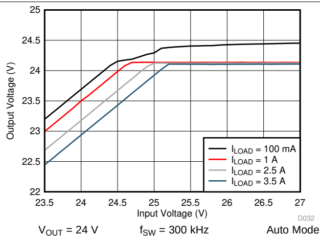
图 57. LM76003 Dropout Curve
