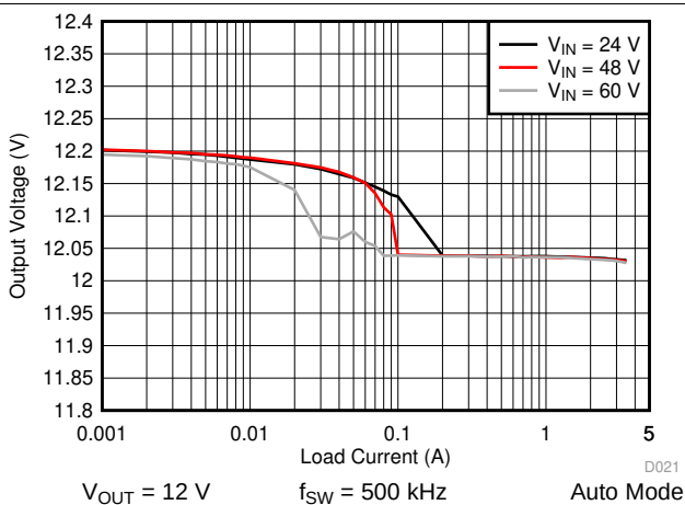
图 45. LM76003 Load and Line Regulation
