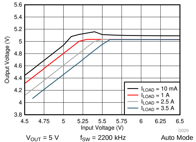
图 54. LM76003 Dropout Curve
