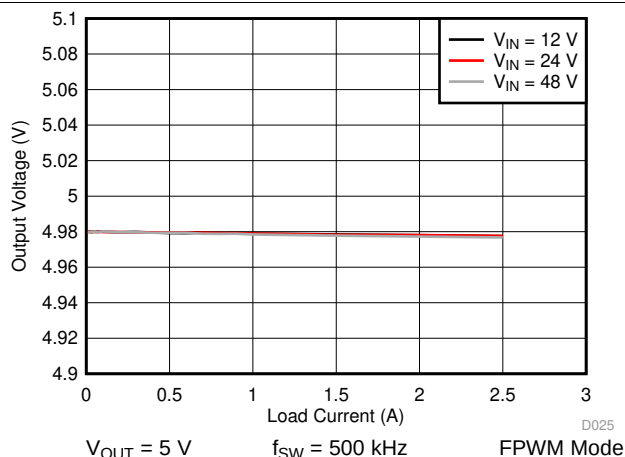
图 50. LM76002 Load and Line Regulation
