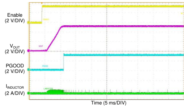
FIG 66. LM76003 Start-up Waveform
