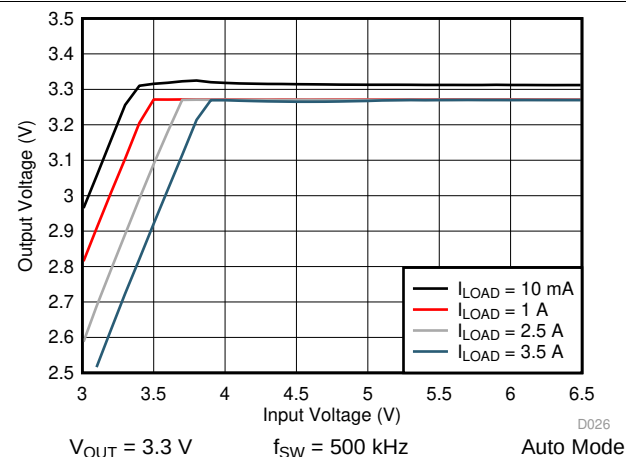
图 51. LM76003 Dropout Curve
