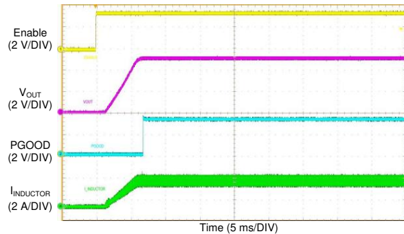
FIG 67. Start-up Waveform
