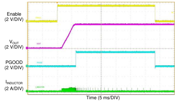
图 62. LM76003 Start-up Waveform
