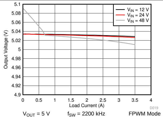
图 44. LM76003 Load and Line Regulation
