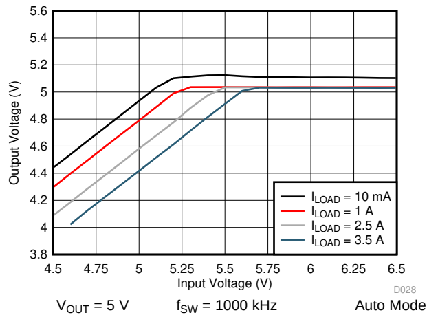
图 53. LM76003 Dropout Curve
