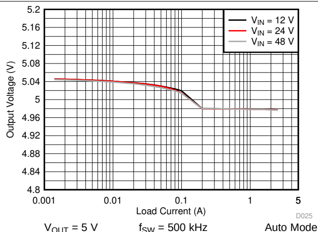
图 49. LM76002 Load and Line Regulation
