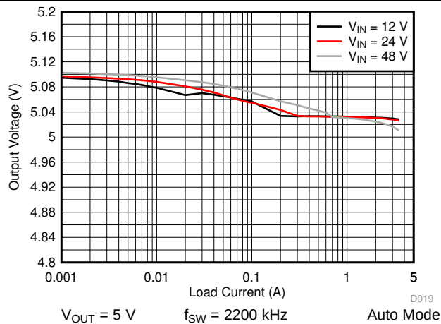
图 43. LM76003 Load and Line Regulation
