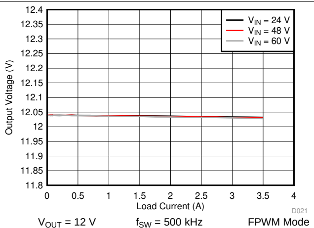
图 46. LM76003 Load and Line Regulation
