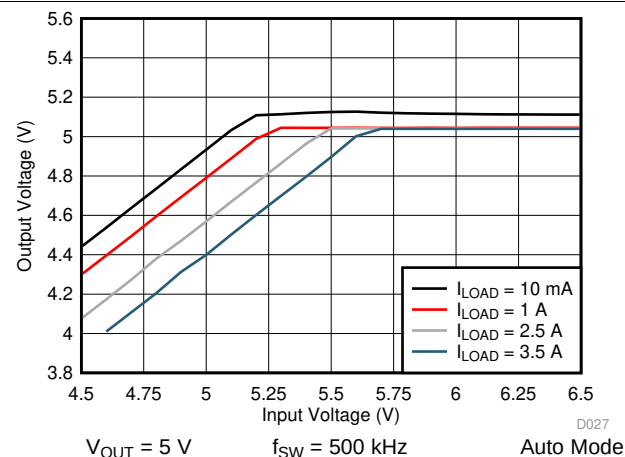
图 52. LM76003 Dropout Curve
