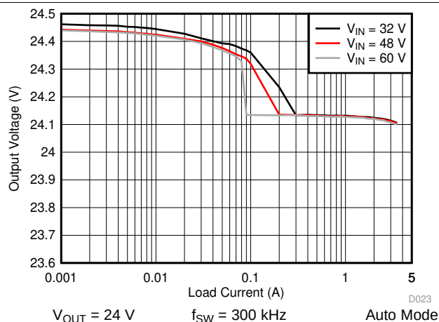
图 47. LM76003 Load and Line Regulation
