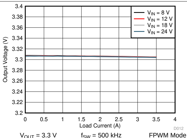
图 38. LM76003 Load and Line Regulation
