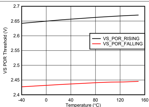
FIG 6-15. VS POR Threshold vs Temperature
