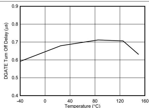
FIG 6-16. DGATE Turn OFF Delay
