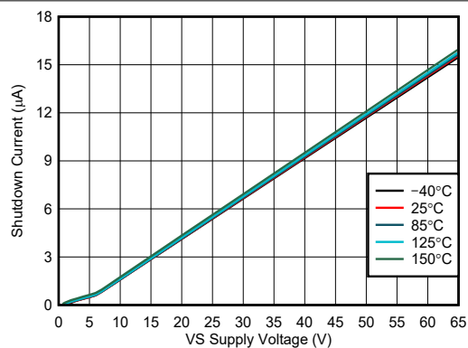
図 6-2. Shutdown Current vs Supply Voltage
