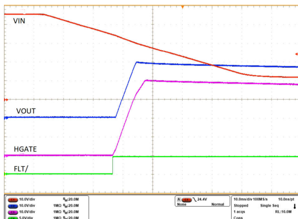
10-15. Overvoltage Recovery
