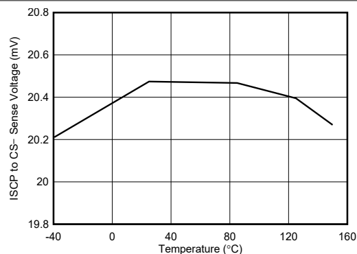
FIG 7-14. ISCP to CS- Threshold vs Temperature
