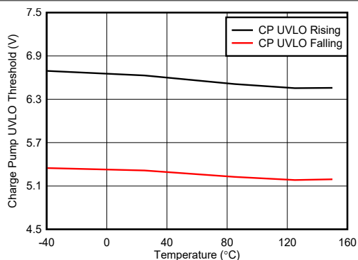
FIG 7-13. Charge Pump UVLO Threshold vs Temperature
