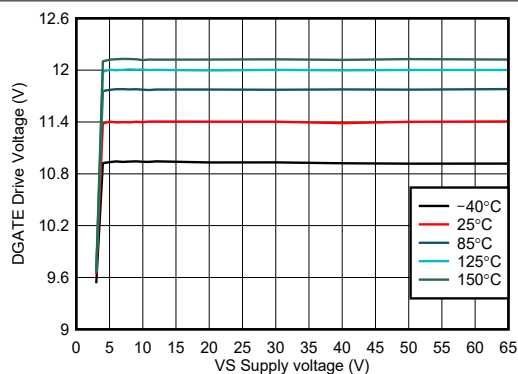
Figure 7-8. DGATE Drive Voltage vs Supply Voltage
