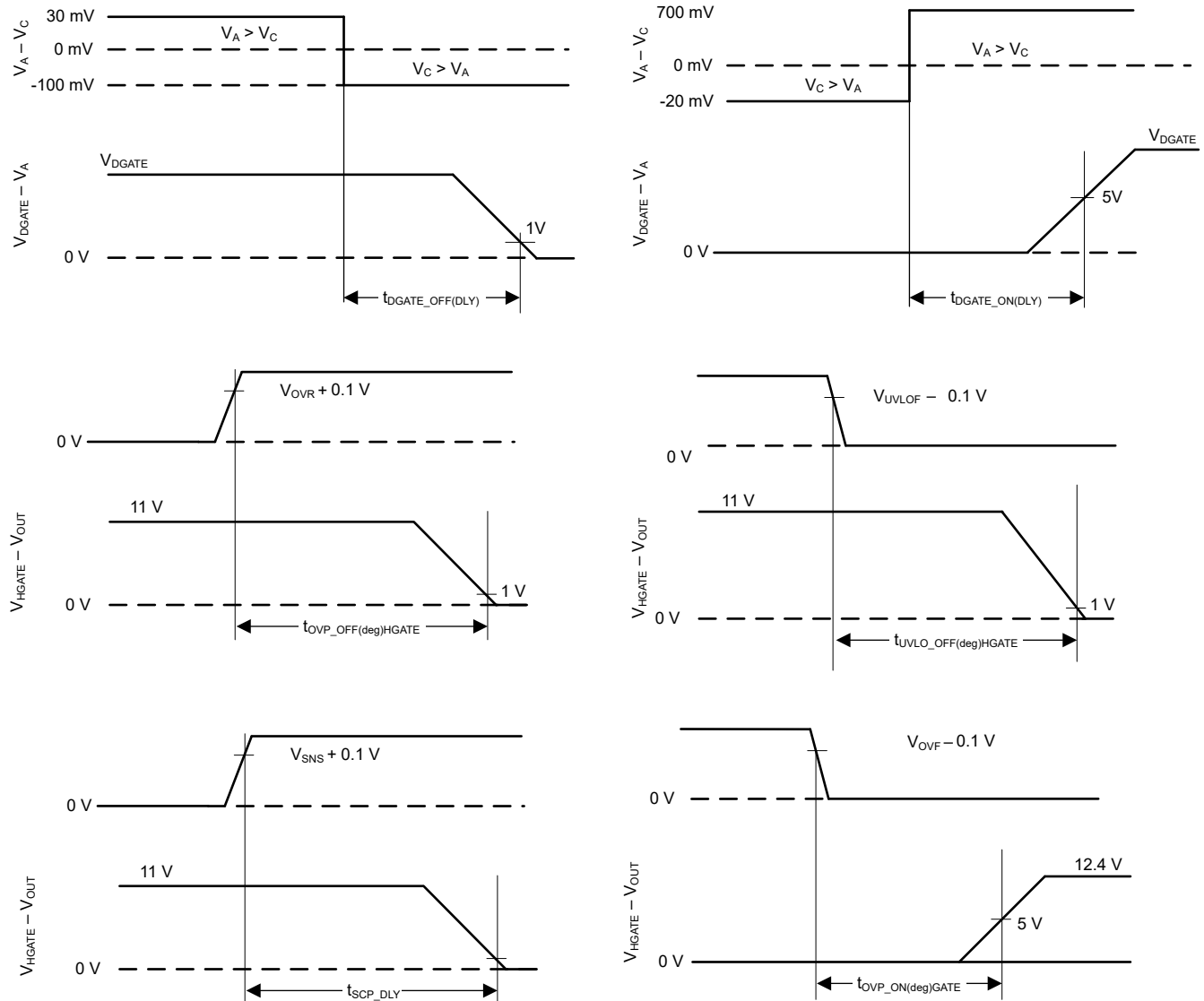
图 8-1. Timing Waveforms
