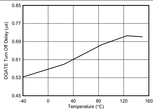
FIG 7-18. DGATE Turn OFF Delay
