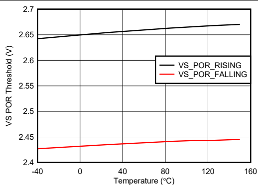
FIG 7-17. VS POR Threshold vs Temperature
