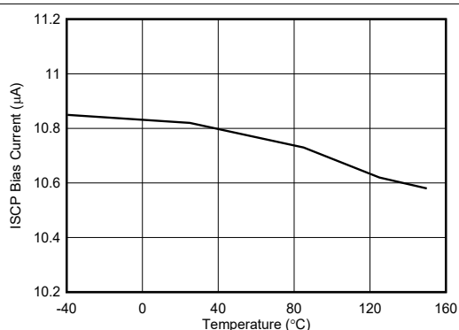
FIG 7-15. ISCP Bias Current vs Temperature
