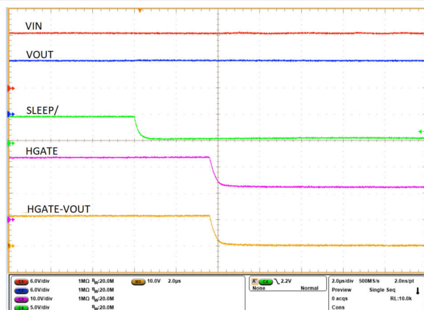
10-19. SLEEP Mode Entry (SLEEP = Low, EN = High)
