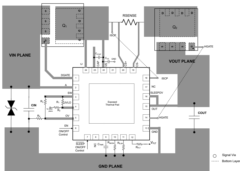
10-24. Example Layout
