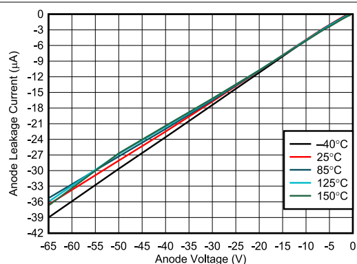
Figure 7-10. ANODE Leakage Current vs Reverse ANODE Voltage
