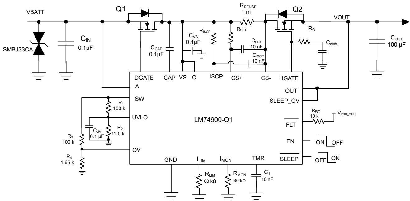
10-1. Typical Application Circuit – 12-V Reverse Battery Protection, Overcurrent Protection, and Overvoltage Protection
