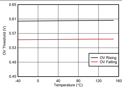
Figure 7-12. OVP Thresholds vs Temperature
