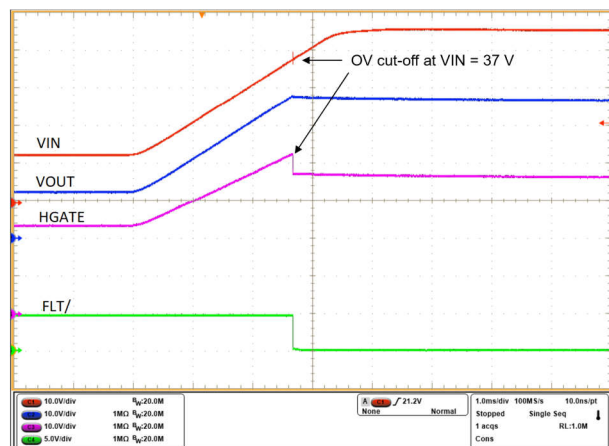
10-14. Overvoltage Protection
