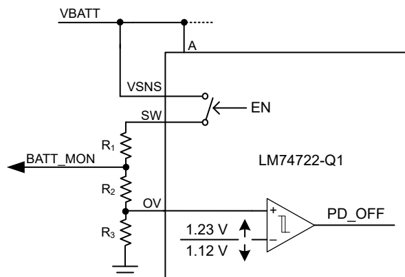
FIG 8-3. Programming Overvoltage Threshold and Battery Voltage Sensing
