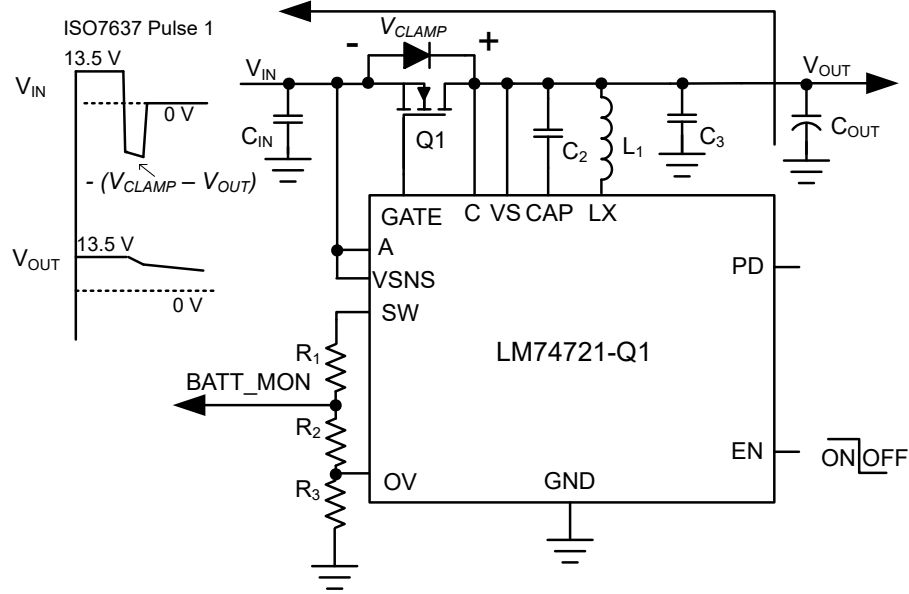
FIG 8-2. LM74721-Q1 Ideal Diode Circuit Operation During ISO7637 Pulse 1
