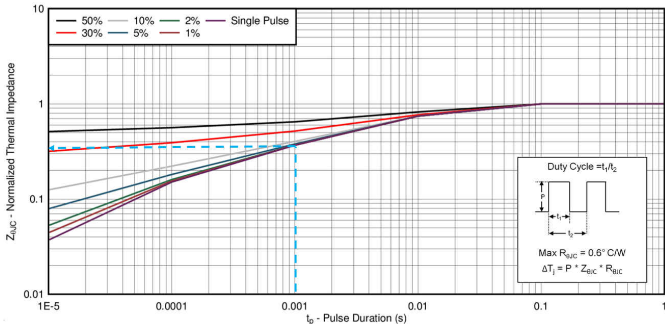
9-3. Typical MOSFET Transient Thermal Impedance
