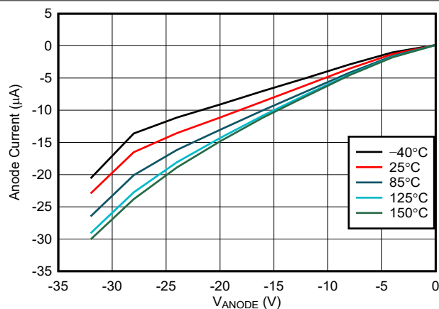
FIG 6-14. Anode Leakage Current vs Reverse Anode Voltage
