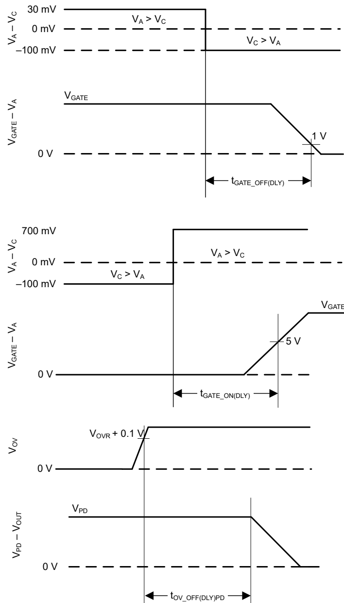
7-1. Timing Waveforms
