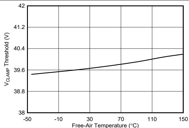
FIG 6-13. V_{CLAMP} vs Temperature
