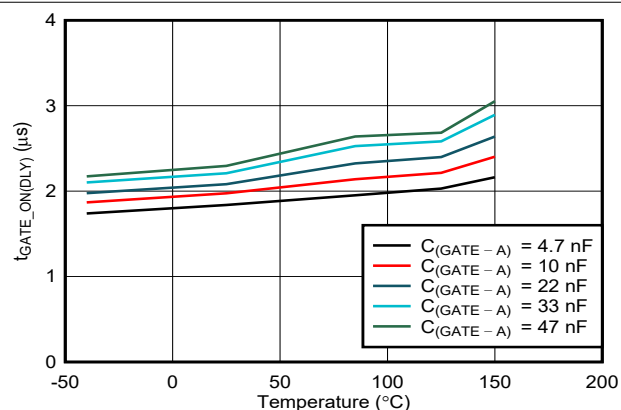
Figure 6-10. Forward Turn-on Delay vs Temperature
