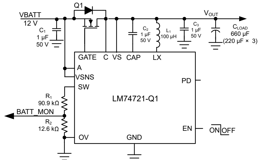
図 9-1. Typical Application Circuit for 12-V TVS-less Reverse Battery Protection
