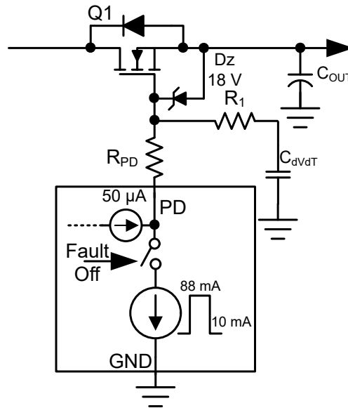
FIG 8-3. Inrush Current Limiting
