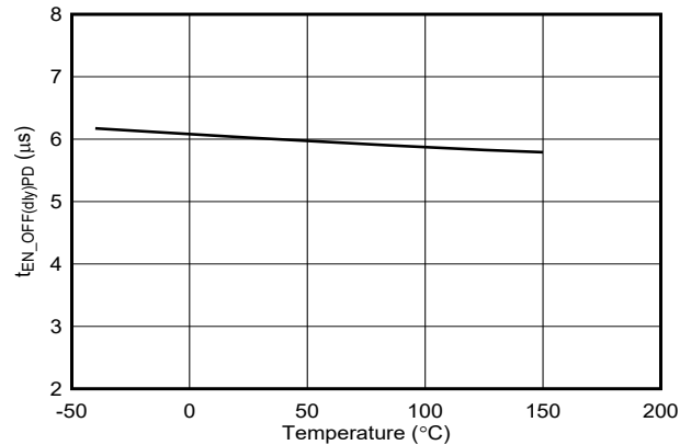
Figure 6-9. PD Turn-off Delay During EN
