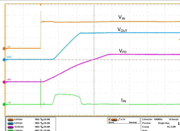
FIG 9-12. Hot-Plug into 12 V
