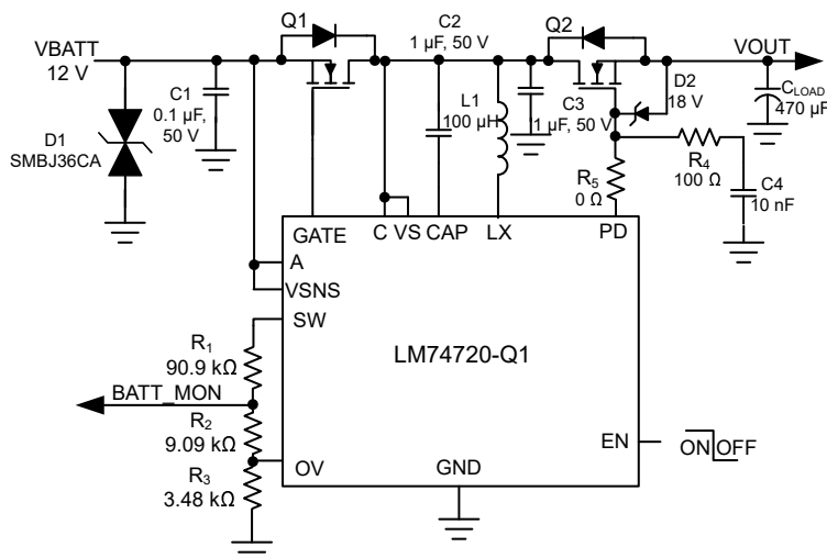
図 9-1. Typical Application Circuit – 12-V Reverse Battery Protection and Overvoltage Protection
