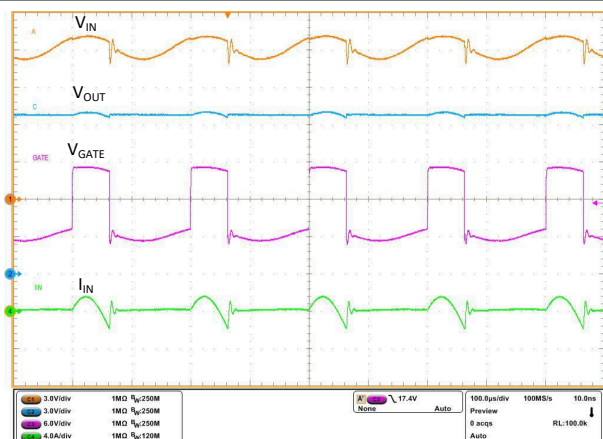
图 9-3. AC Super Imposed Test – 2-V Peak-Peak 5 kHz
