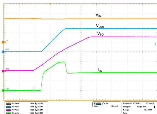
FIG 9-11. Inrush Current with 60- \Omega Load
