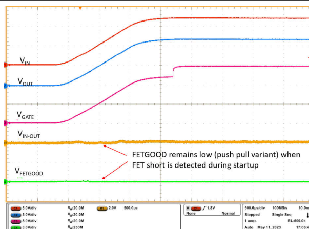
9-7. Start-up With 5.8-A Load
