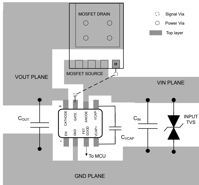
9-14. LM74703-Q1 DDF Package Example Layout
