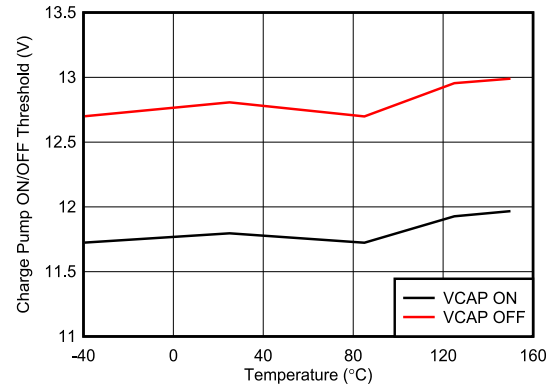
図 6-14. Charge Pump ON/OFF Threshold vs Temperature
