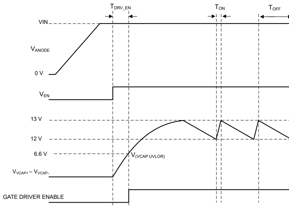
図 8-1. Charge Pump Operation
