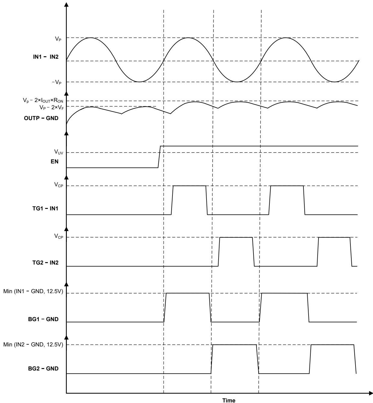
7-2. Enable Response and Gate Drivers Operation
