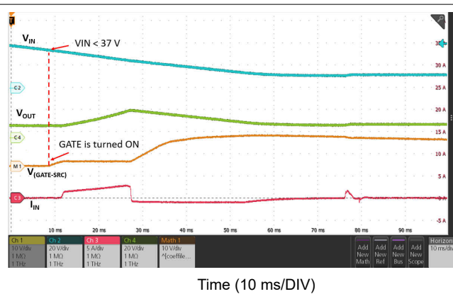
9-7. Overvoltage Recovery
