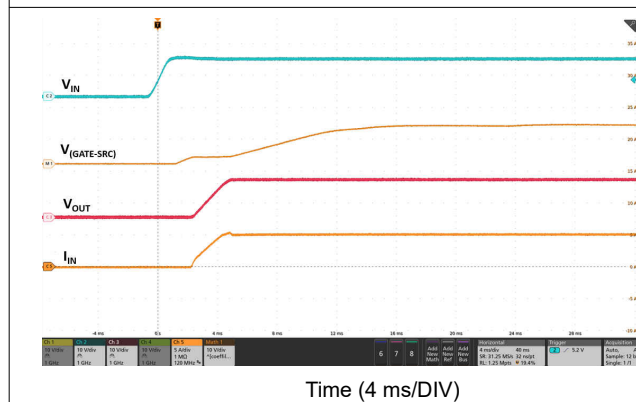
9-4. Start-up with 5-A Load
