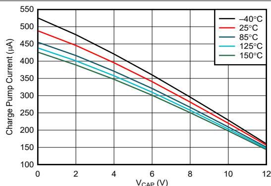
FIG 6-4. Charge Pump V-I Characteristics at V_S \geq 12\text{ V}
