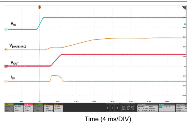
9-3. Start-up with No Load
