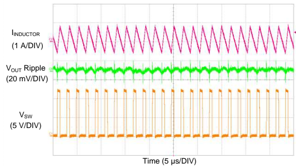
図 58. LM73606 Switching Waveform and V_{OUT} Ripple
