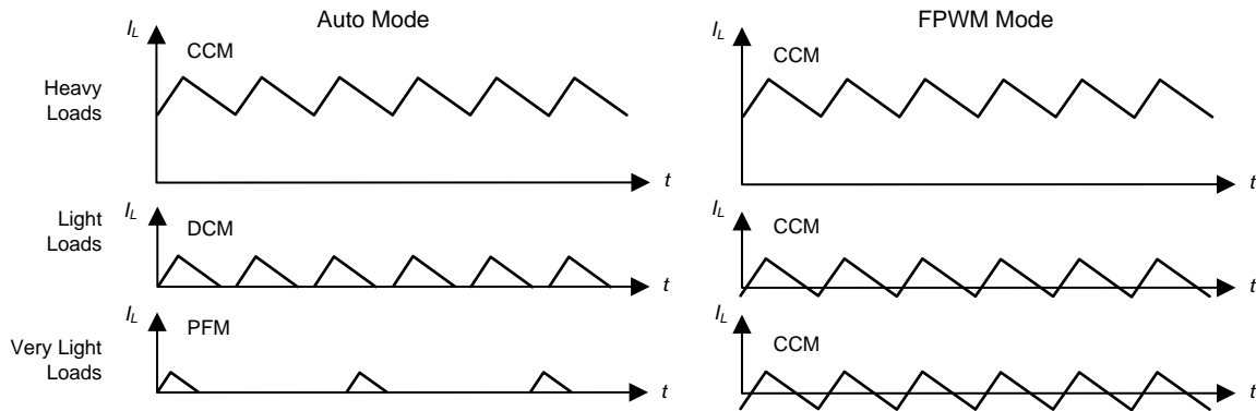
図 11. Inductor Current Waveforms at Auto Mode and FPWM Mode with Different Loads
