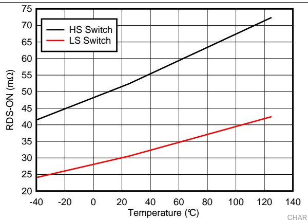
図 1. High-Side and Low-Side Switches R_{DS-ON}
