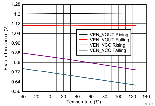
FIG 8. Enable Thresholds
