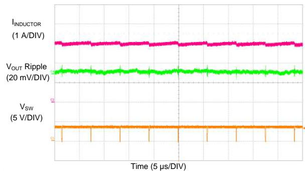
図 60. LM73606 Switching Waveform and V_{OUT} Ripple
