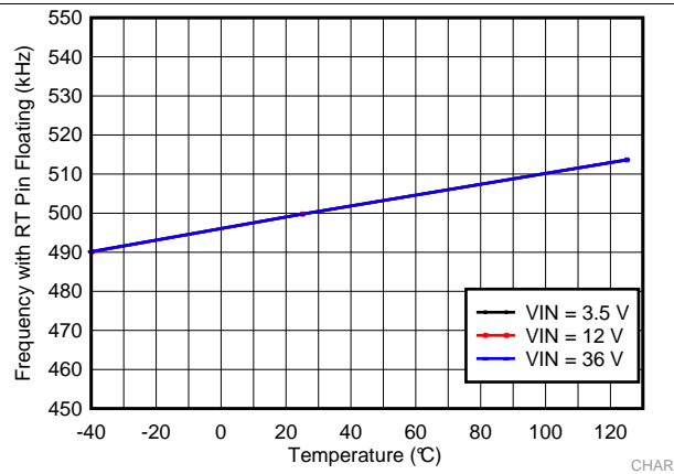
FIG 7. Switching Frequency with RT Pin Open Circuit
