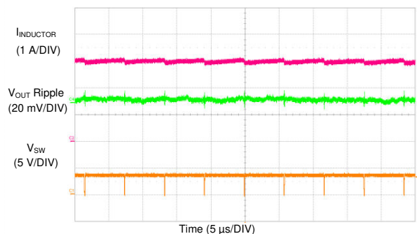
FIG 9-48. LM73606-Q1 Switching Waveform and V_{\text{OUT}} Ripple
