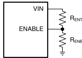
Figure 8-5. System UVLO
