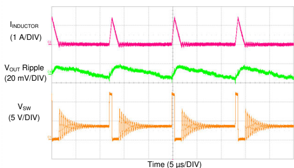
FIG 9-45. LM73606-Q1 Switching Waveform and V_{\text{OUT}} Ripple
