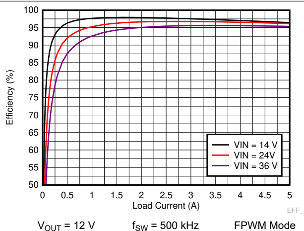
9-20. LM73605-Q1 Efficiency
