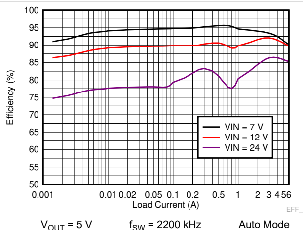
9-17. LM73606-Q1 Efficiency
