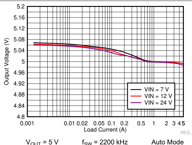
FIG 9-25. LM73605-Q1 Load and Line Regulation
