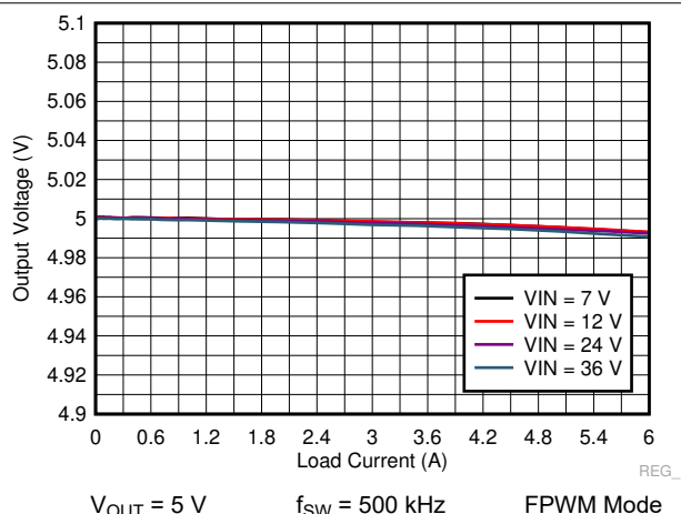
FIG 9-24. LM73606-Q1 Load and Line Regulation
