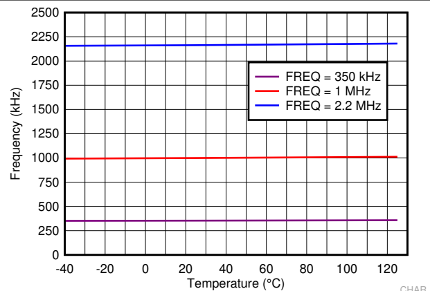
7-6. Switching Frequency Set by R_T Resistor
