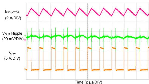
FIG 9-47. LM73606-Q1 Switching Waveform and V_{\text{OUT}} Ripple
