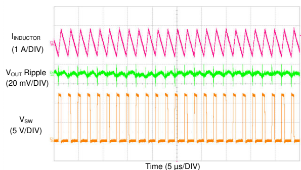
FIG 9-46. LM73606-Q1 Switching Waveform and V_{\text{OUT}} Ripple
