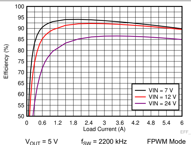
9-18. LM73606-Q1 Efficiency
