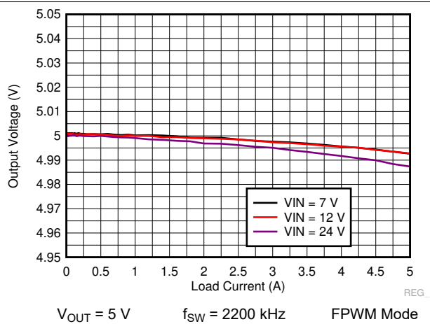
FIG 9-26. LM73605-Q1 Load and Line Regulation
