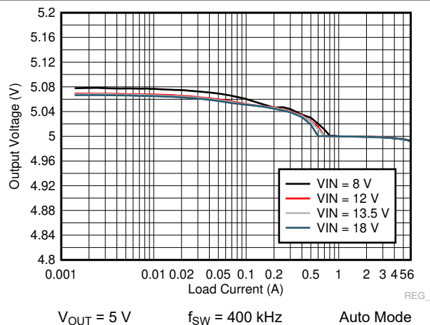
FIG 9-21. LM73606-Q1 Load and Line Regulation
