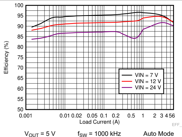
9-15. LM73606-Q1 Efficiency
