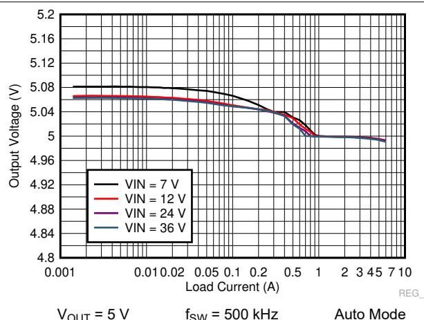
FIG 9-23. LM73606-Q1 Load and Line Regulation
