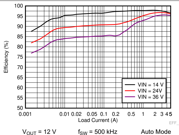
9-19. LM73605-Q1 Efficiency
