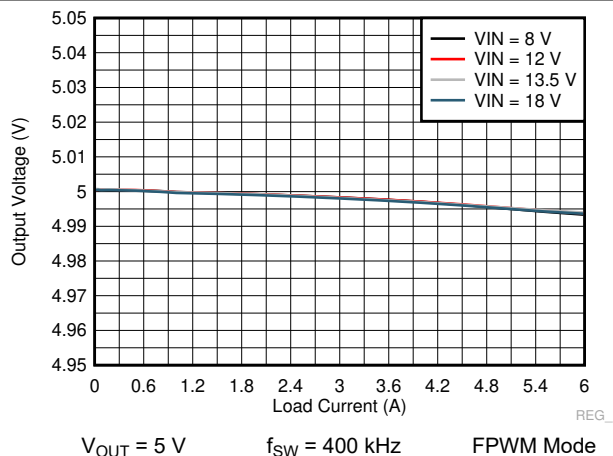
FIG 9-22. LM73606-Q1 Load and Line Regulation
