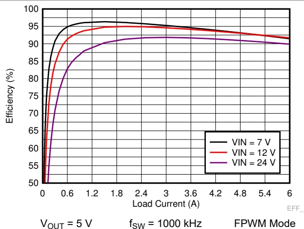
9-16. LM73606-Q1 Efficiency
