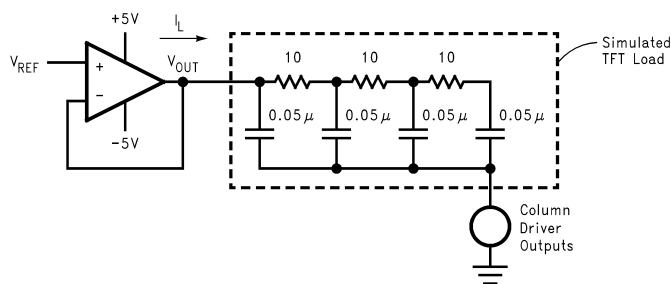
Figure 67. V_{COM} Driver Application Schematic
