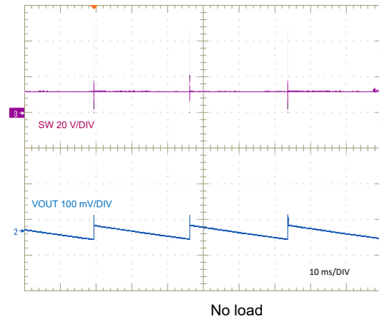
7-23. PFM Switching
