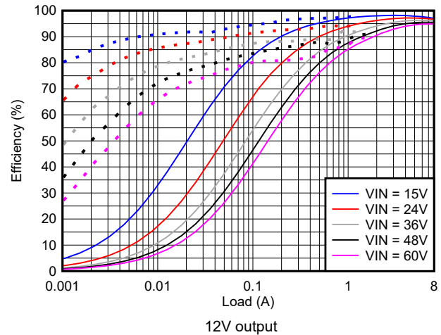
7-21. Efficiency versus I_{OUT} , Log Scale
