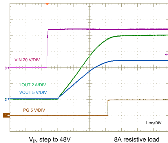
7-24. Start-Up Characteristic
