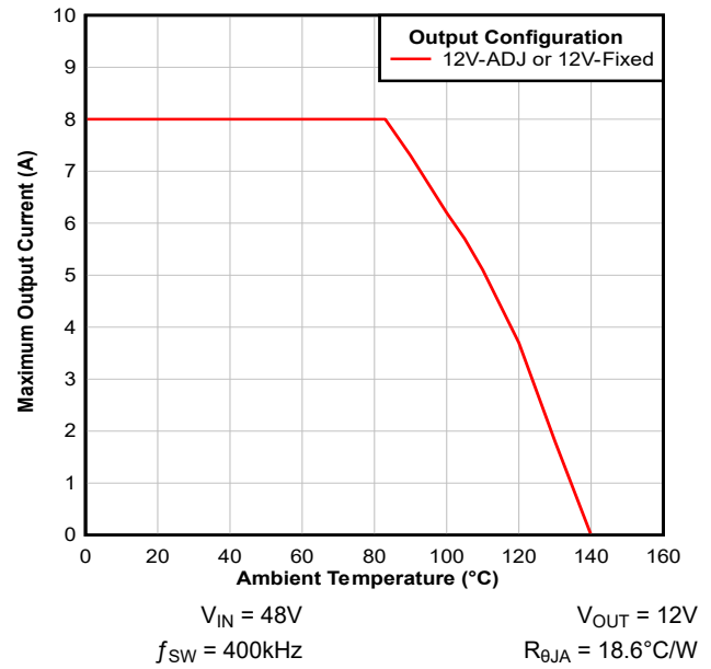
7-7. Maximum Output Current versus Ambient Temperature
