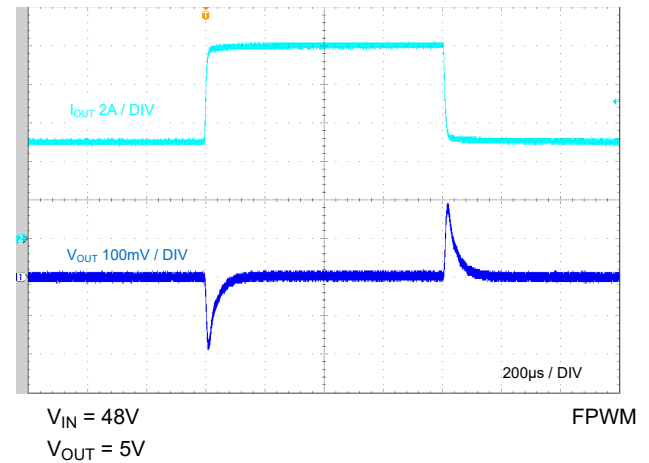
図 5-10. Load Transient, 5A to 10A
