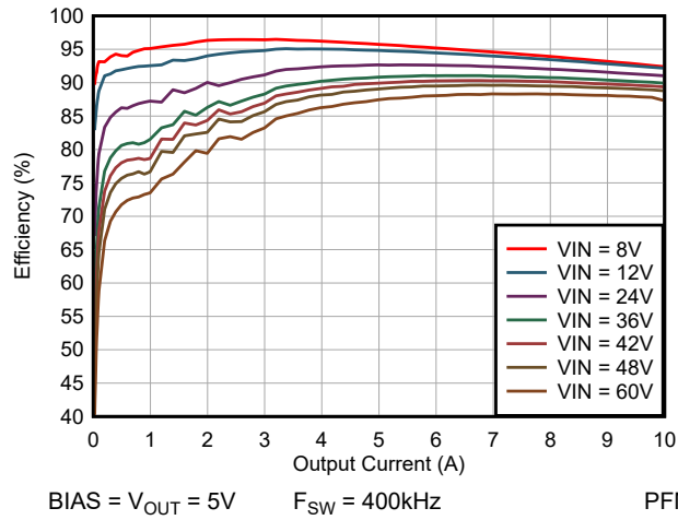
図 5-7. Efficiency vs I_{OUT} , Linear Scale
