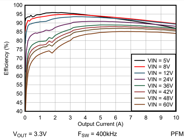
7-26. Efficiency versus I_{OUT} , Linear Scale
