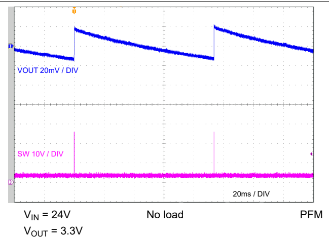
7-29. PFM Switching
