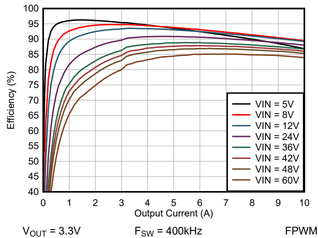
7-24. Efficiency versus I_{OUT} , Linear Scale
