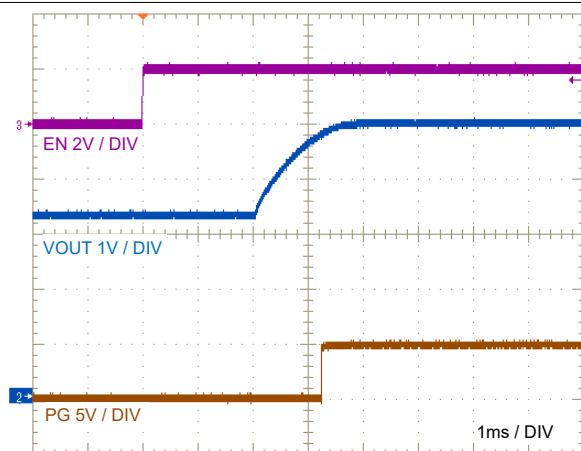
図 7-17. Start-Up Characteristic
