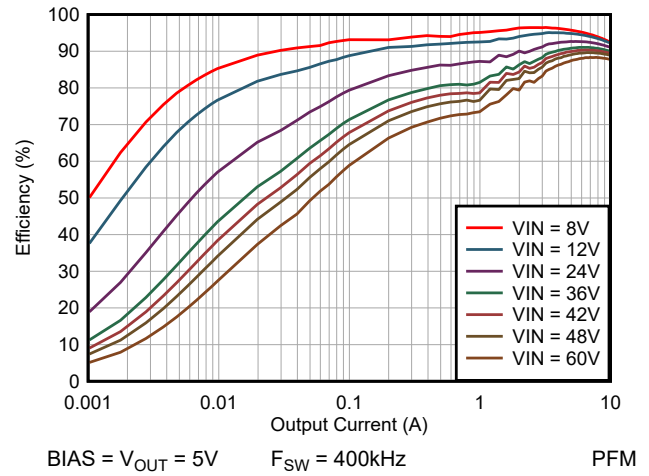
図 5-8. Efficiency vs I_{OUT} , Log Scale
