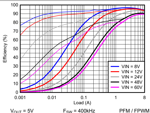
図 7-14. Efficiency versus I_{OUT} , Log Scale
