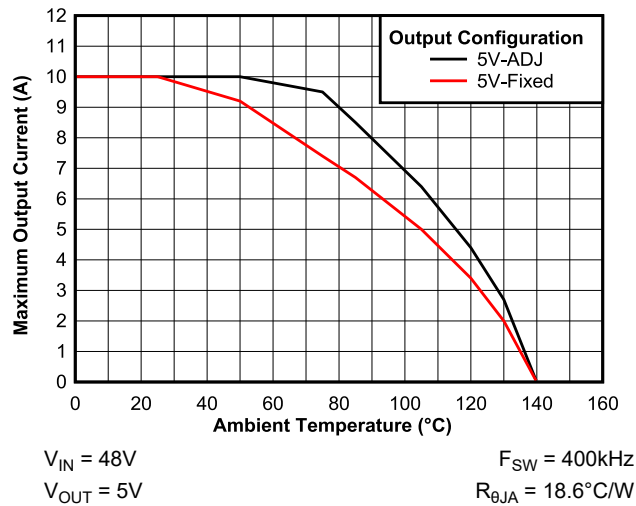
7-8. Maximum Output Current versus Ambient Temperature
