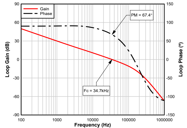
V_{IN} = 24V F_{SW} = 400kHz FPWM V_{OUT} = 3.3V I_{OUT} = 10A (resistive) L = 2.2\mu H
