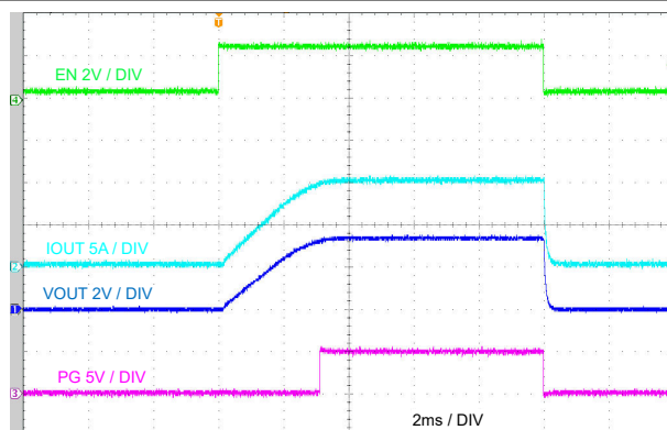
図 7-27. EN Start-Up and Shutdown Characteristic
