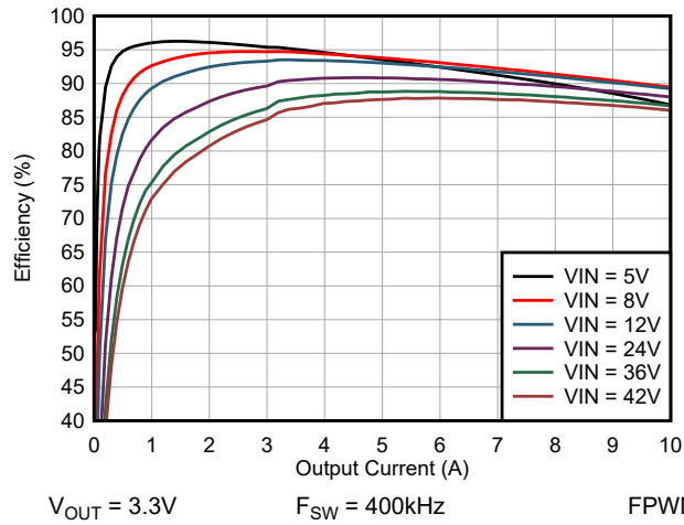
Figure 5-1. Efficiency vs I_{OUT} , Linear Scale
