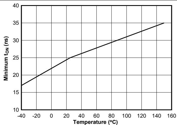
图 5-14. Minimum On-Time vs Temperature
