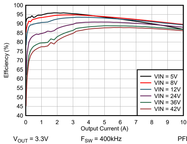
Figure 5-3. Efficiency vs I_{OUT} , Linear Scale
