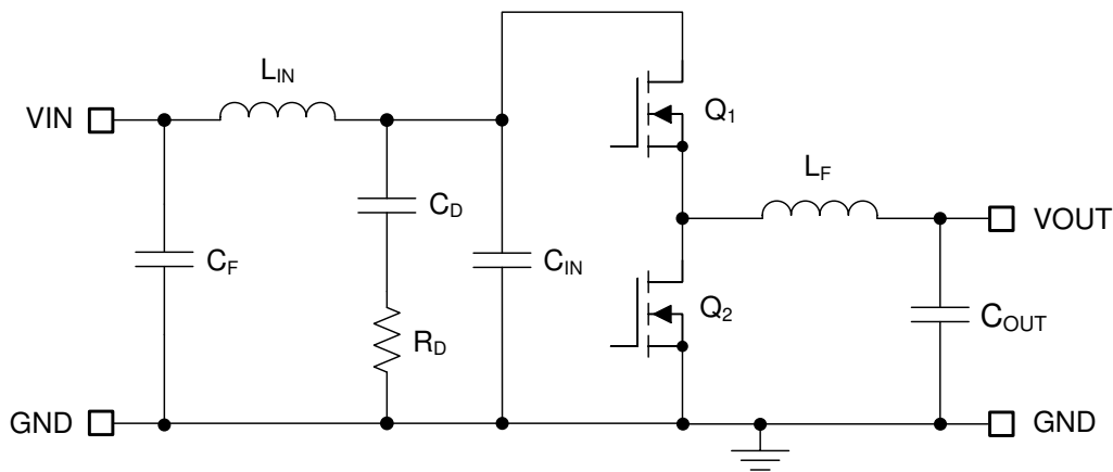
図 7-2. Buck Regulator With π-Stage EMI Filter
