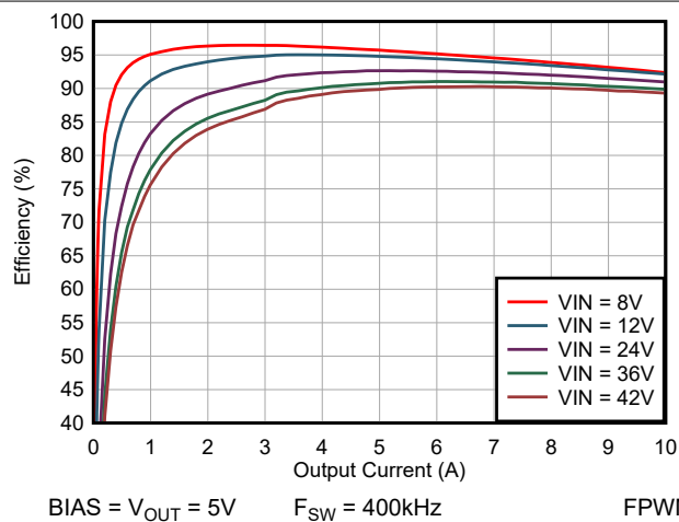
Figure 5-5. Efficiency vs I_{OUT} , Linear Scale
