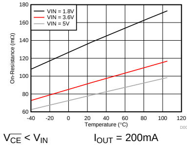
图 4. On-Resistance vs Junction Temperature
