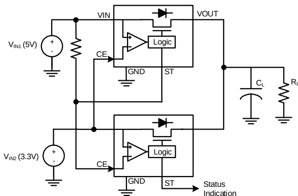
FIG 17. Dual Ideal Diode ORing for Continuous Output Power
