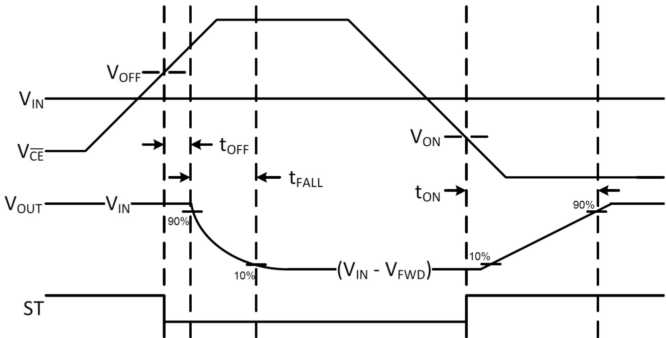
Figure 11. Timing Diagram
