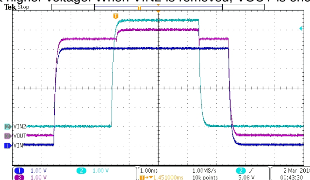
FIG 16. Dual Ideal Diode ORing Behavior
