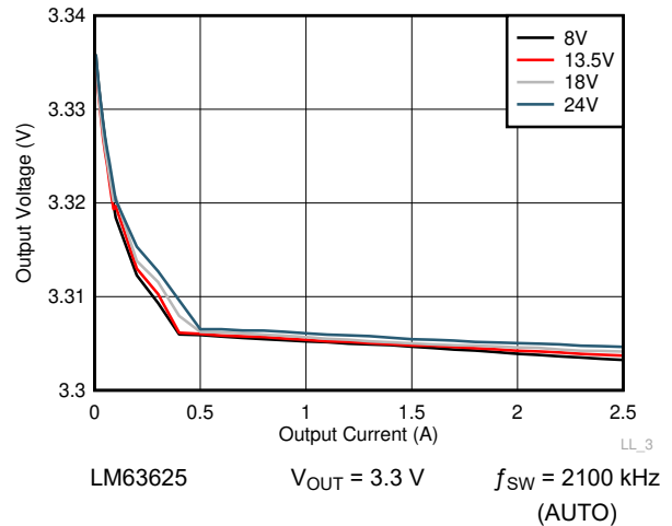
図 8-17. Line and Load Regulation
