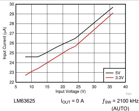
図 8-38. Input Supply Current versus Input Voltage
