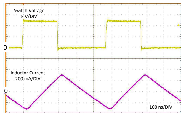
図 7-7. Typical PWM Switching Waveforms Without Spread Spectrum V_{IN} = 12 V, V_{OUT} = 5 V, I_{OUT} = 2.5 A, f_{SW} = 2100 kHz
