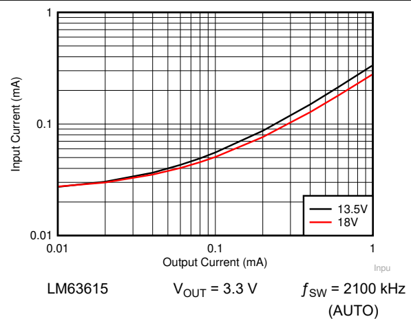
図 8-43. Input Supply Current versus Output Current
