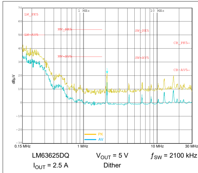
Figure 8-45. Typical Conducted EMI 0.15 MHz to 30 MHz
