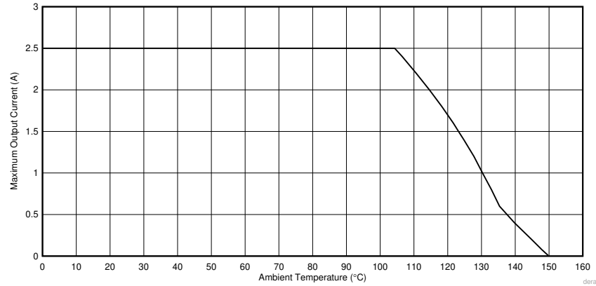
図 8-6. Maximum Output Current versus Ambient Temperature V_{IN} = 12\text{ V} , V_{OUT} = 5\text{ V} , f_{SW} = 2.1\text{ MHz} , R_{\theta JA} = 30^\circ\text{C/W}
