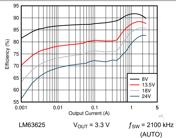
図 8-13. Efficiency
