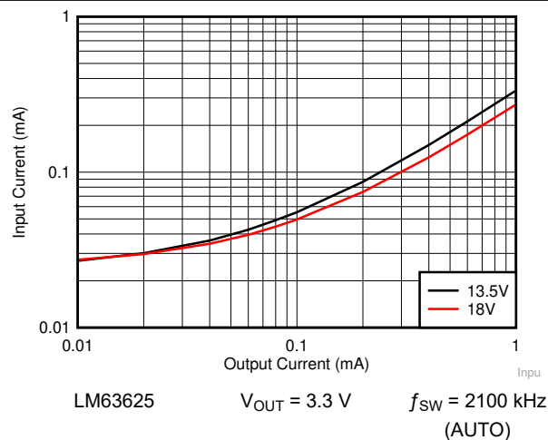
図 8-42. Input Supply Current versus Output Current
