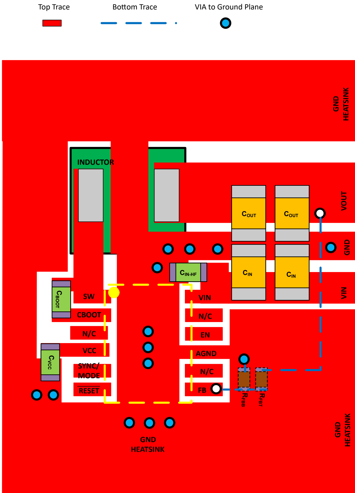
図 8-51. Example Layout for WSON Package 2nd pinout
