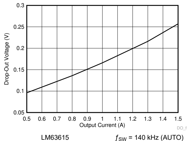
図 8-36. Dropout Voltage versus Output Current for -1% Drop
