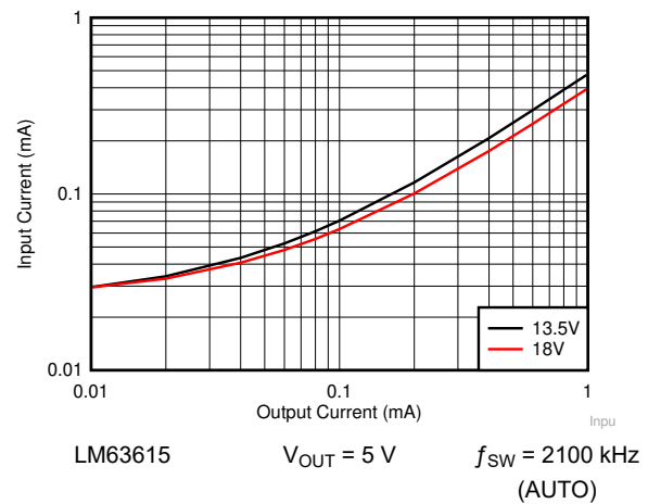
図 8-41. Input Supply Current versus Output Current
