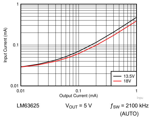
図 8-40. Input Supply Current versus Output Current
