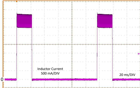
7-12. Inductor Current Burst in Short-Circuit Mode; LM63625
