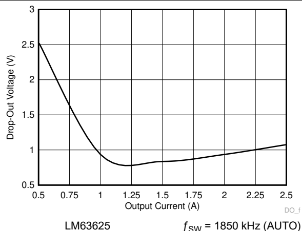
図 8-35. Dropout Voltage versus Output Current to 1.85 MHz
