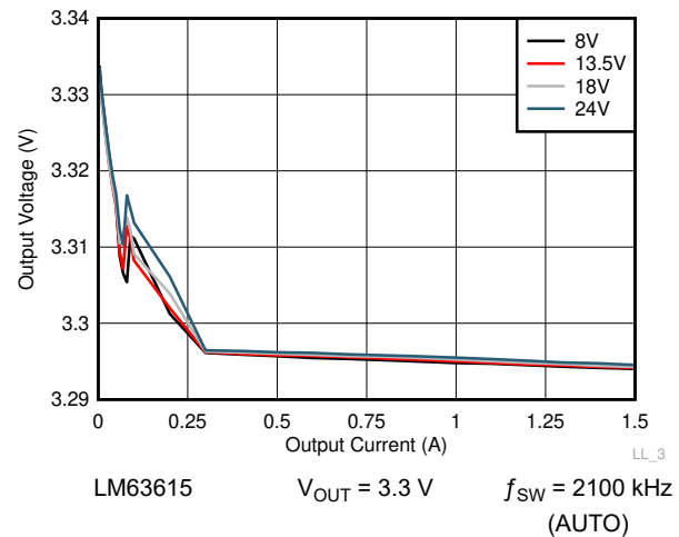
図 8-19. Line and Load Regulation
