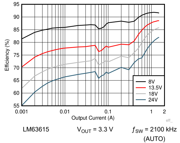
図 8-15. Efficiency
