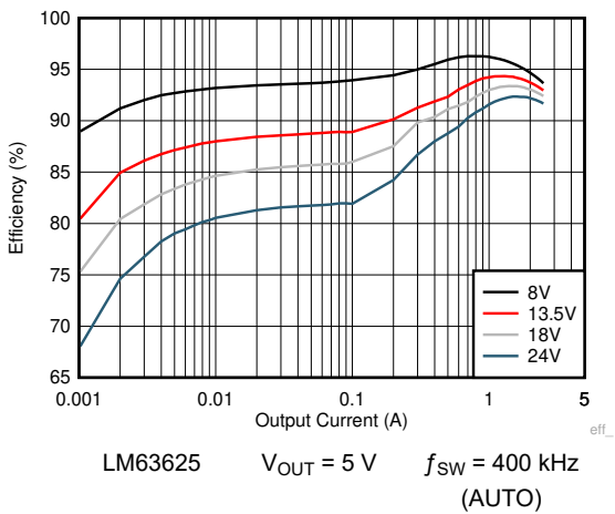
図 8-8. Efficiency
