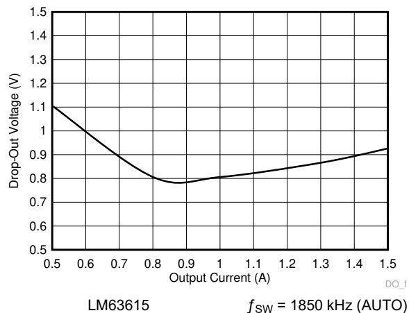
図 8-37. Dropout Voltage versus Output Current to 1.85 MHz
