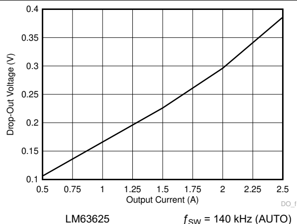
図 8-34. Dropout Voltage versus Output Current for -1% Drop
