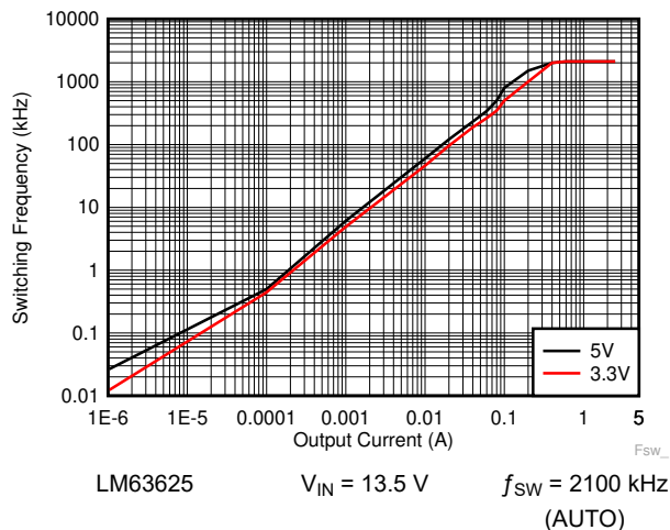
図 8-20. Switching Frequency versus Output Current
