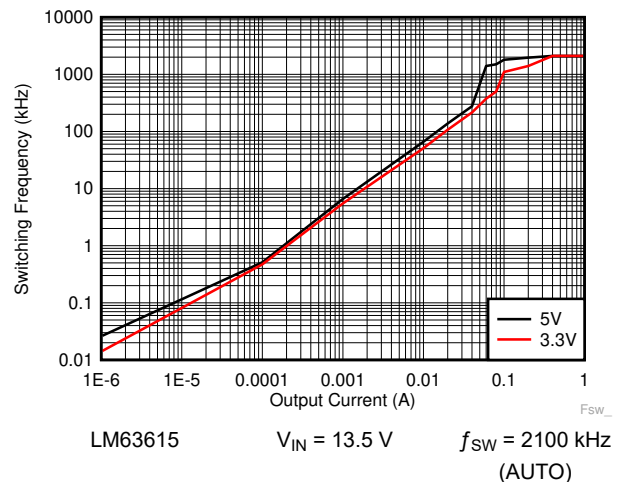
図 8-21. Switching Frequency versus Output Current
