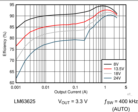
図 8-12. Efficiency
