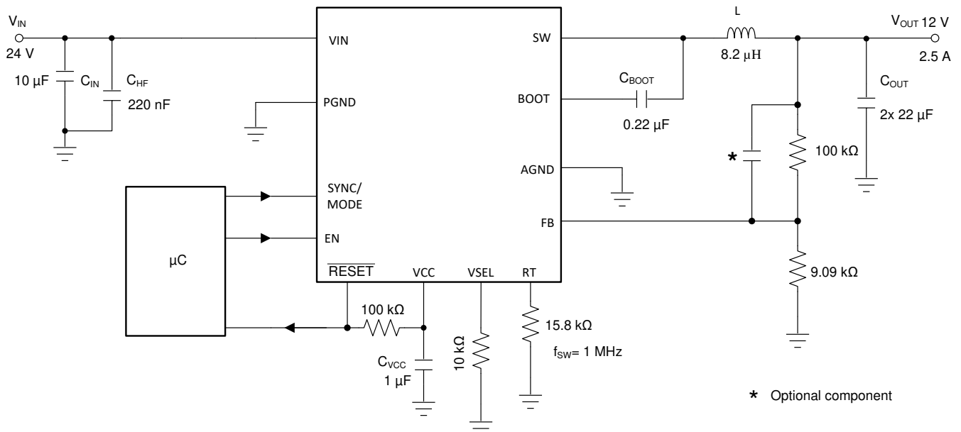
図 8-7. Full-Featured Design Example V_{IN} = 24\text{ V} , V_{OUT} = 12\text{ V} , I_{OUT} = 2.5\text{ A} , f_{SW} = 1\text{ MHz}
