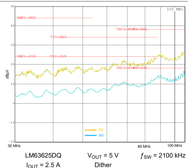
Figure 8-46. Typical Conducted EMI 30 MHz to 108 MHz
