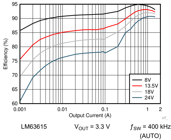
図 8-14. Efficiency
