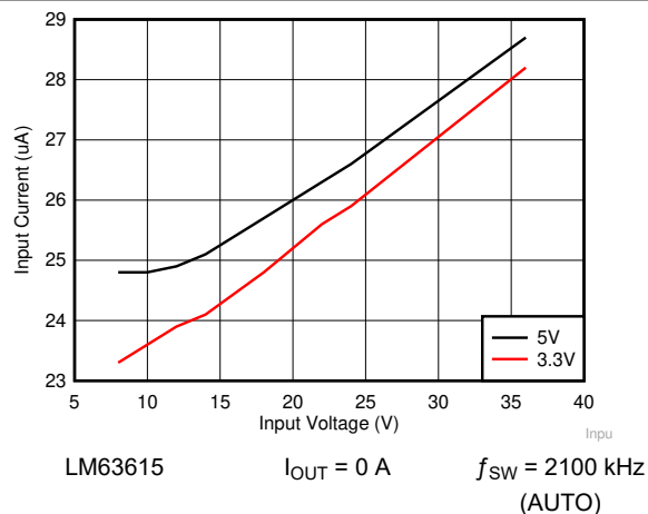
図 8-39. Input Supply Current versus Input Voltage
