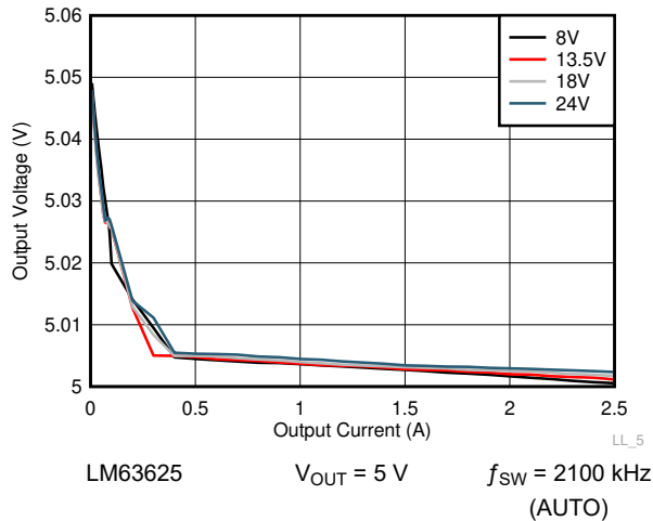
図 8-16. Line and Load Regulation
