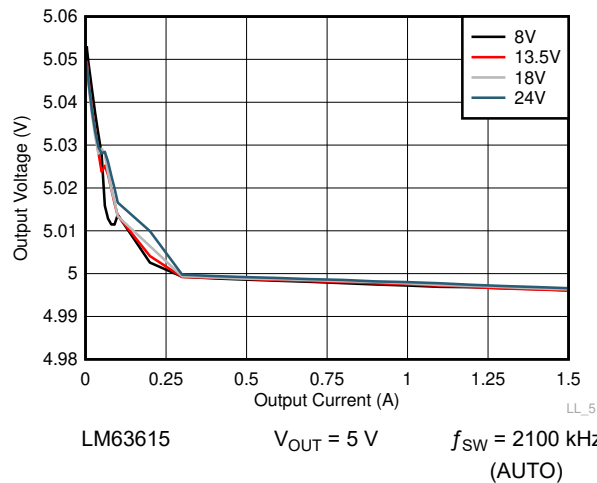
図 8-18. Line and Load Regulation
