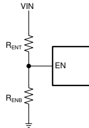
図 8-3. Setup for External UVLO Application
