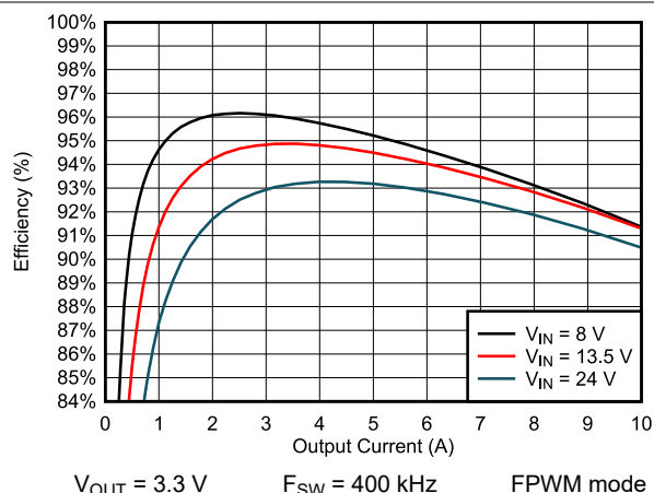
Figure 9-8. Efficiency
