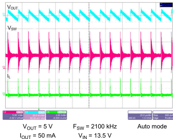
图 9-29. Switching Waveform and V_{OUT} Ripple
