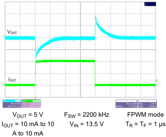
9-43. Load Transient
