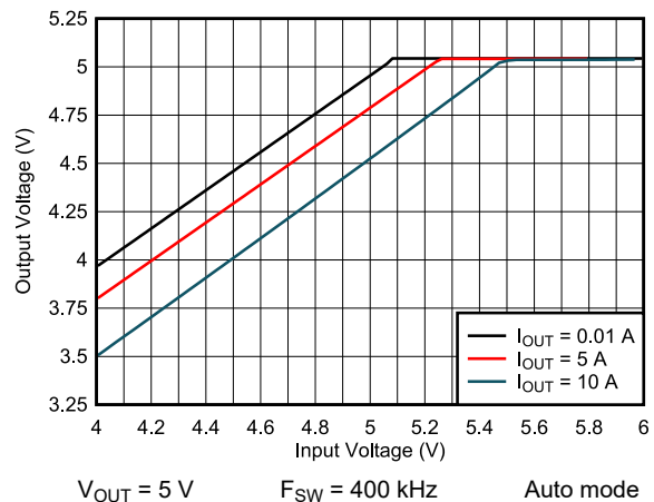
Figure 9-21. Dropout
