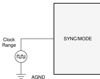
FIG 8-3. Typical Implementation Allowing Synchronization Using the SYNC/MODE Pin
