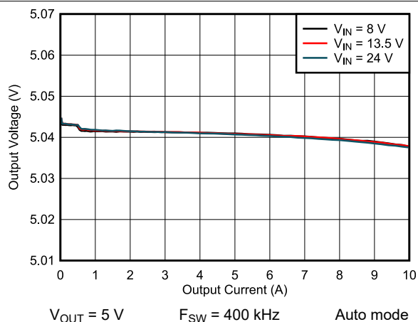
9-13. Load and Line Regulation
