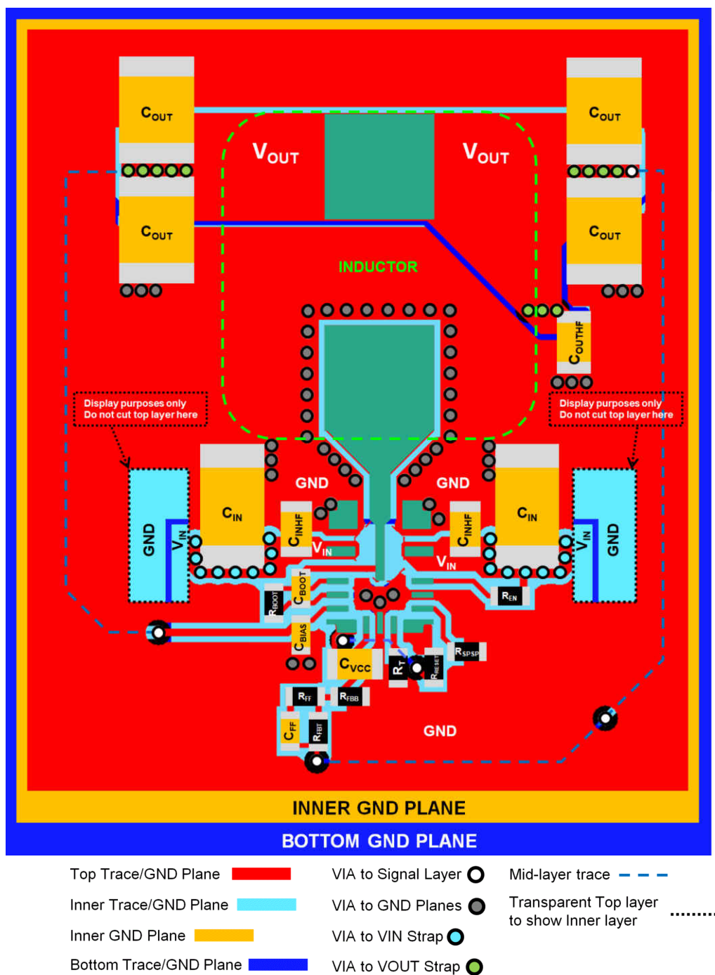
☒ 11-2. Layout Example
