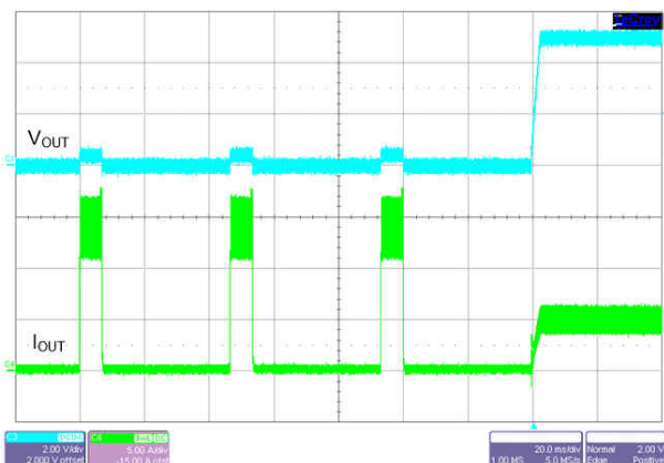
图 9-35. Short Circuit Recovery
