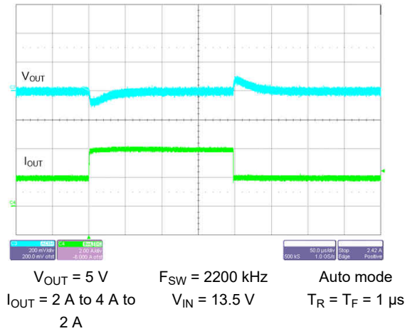
9-44. Load Transient
