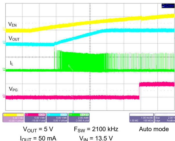
图 9-31. Start-up with 50-mA Load
