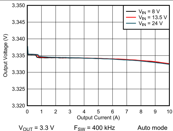
9-15. Load and Line Regulation
