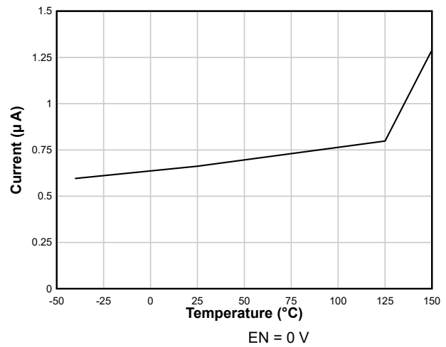
7-2. Shutdown Supply Current
