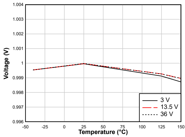
7-1. Feedback Voltage
