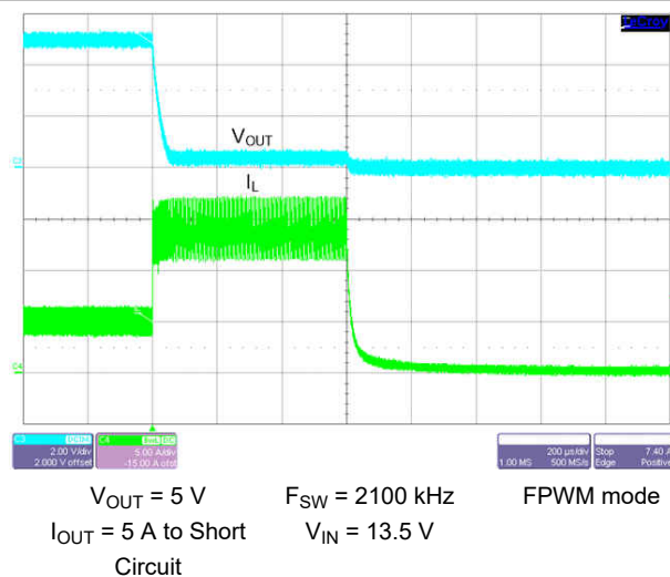
图 9-34. Short Circuit Protection
