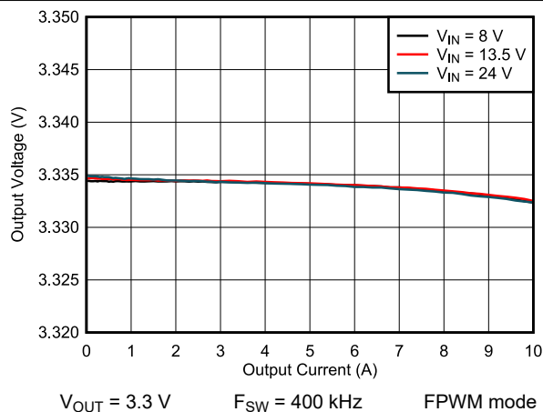
9-16. Load and Line Regulation
