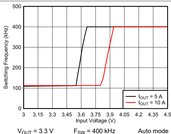
9-26. Frequency Dropout
