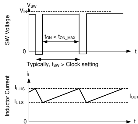
図 8-16. Current Limit Waveforms
