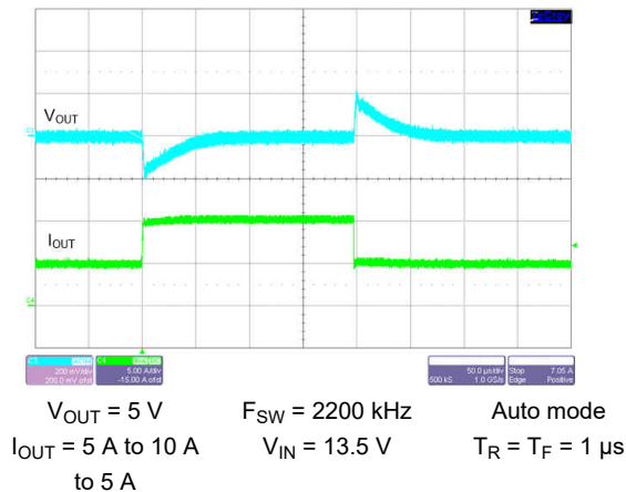
9-45. Load Transient
