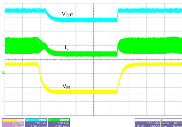
图 9-36. Recovery from Dropout
