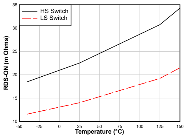
7-3. High-side and Low-side Switches R_{DS\_ON}
