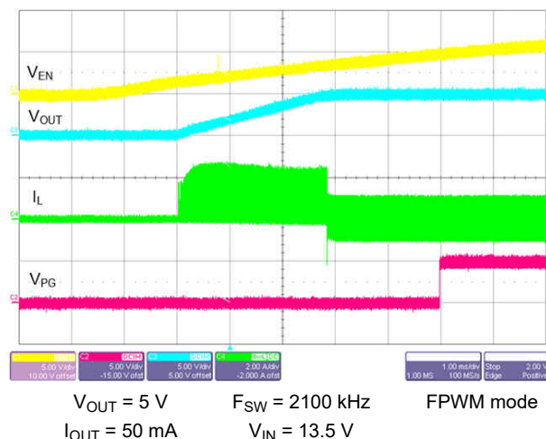
图 9-32. Start-up with 50-mA Load
