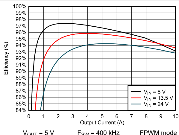
Figure 9-6. Efficiency
