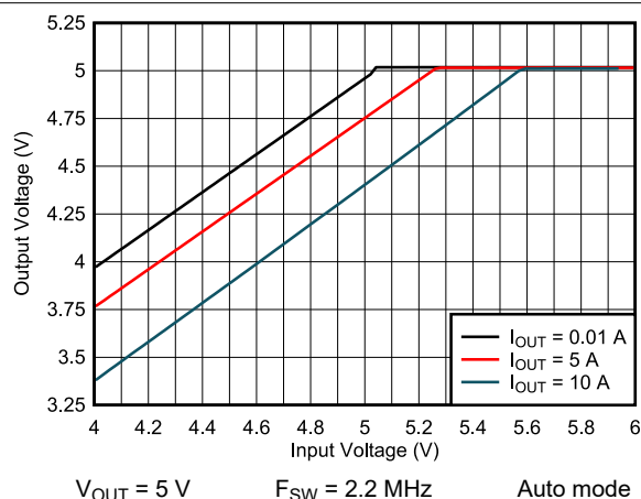
9-23. Dropout
