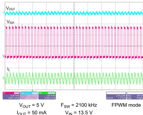
图 9-30. Switching Waveform and V_{OUT} Ripple
