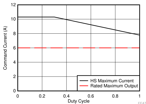
8-15. Maximum Current Allowed Through the HS FET - Function of Duty Cycle for LM62460-Q1
