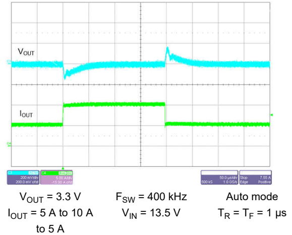
9-42. Load Transient
