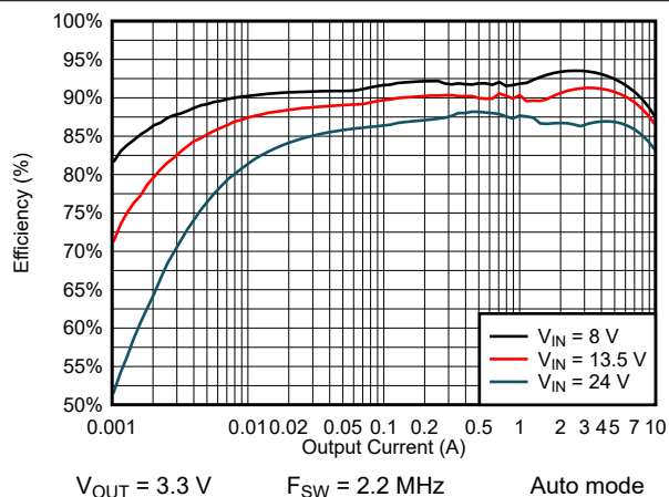
9-11. Efficiency
