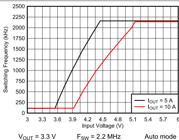
9-28. Frequency Dropout
