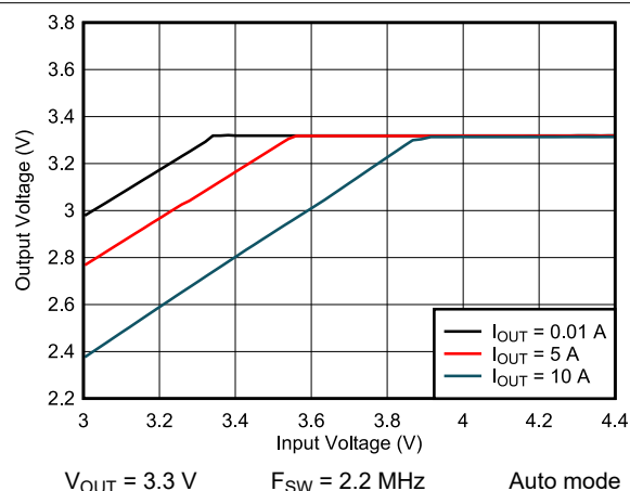
9-24. Dropout
