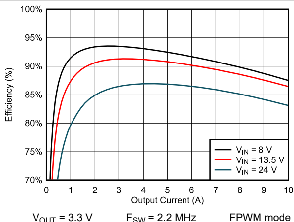
9-12. Efficiency
