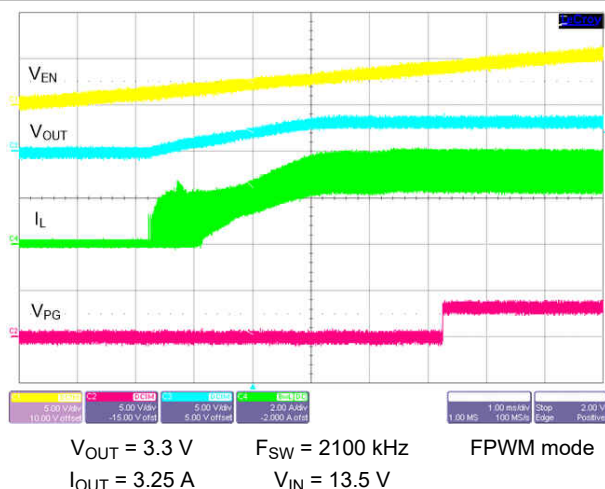
图 9-33. Start-up with 3.25-A Load
