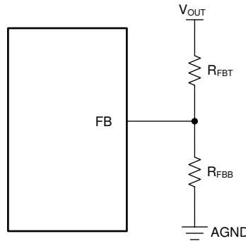
Figure 8-1. Setting Output Voltage of Adjustable Versions
