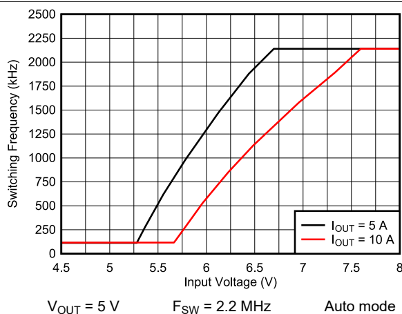
9-27. Frequency Dropout
