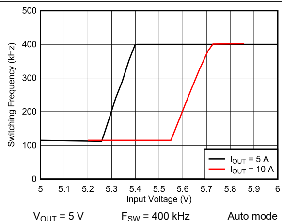
9-25. Frequency Dropout
