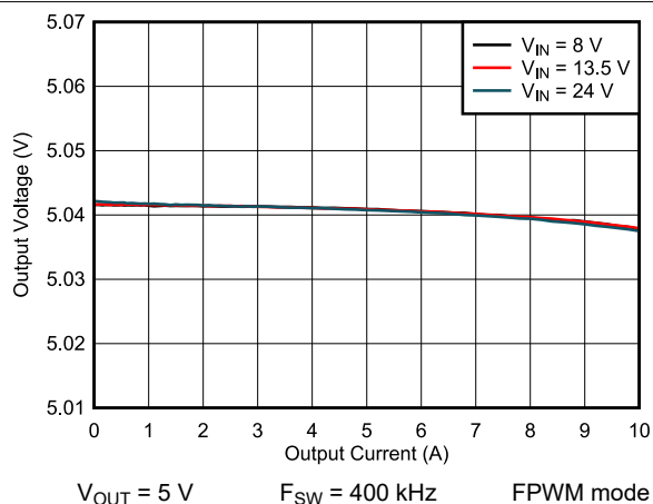
9-14. Load and Line Regulation
