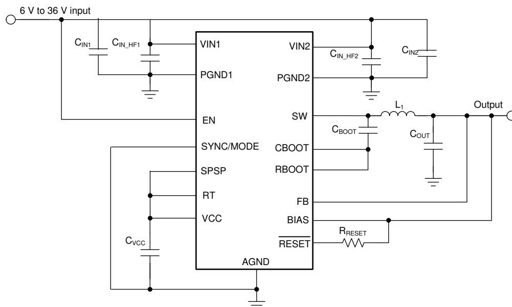
9-2. Example Application Circuit - 400-kHz Fixed Output
