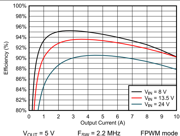
Figure 9-10. Efficiency
