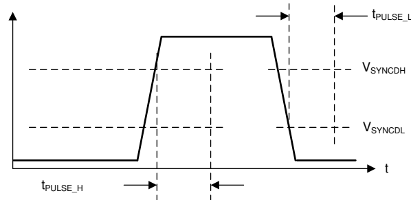
8-4. Typical SYNC/MODE Waveform
