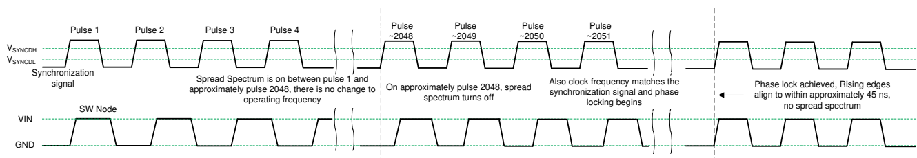
图 8-12. Synchronization Process
