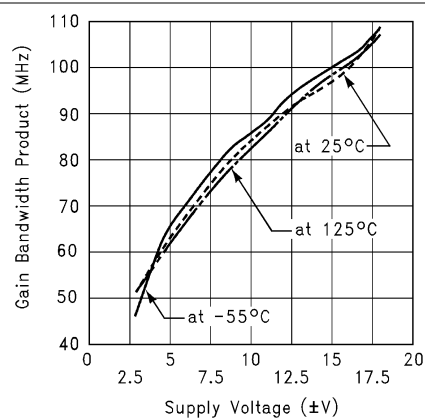
图 5-53. Gain-Bandwidth Product vs Supply Voltage at Different Temperature
