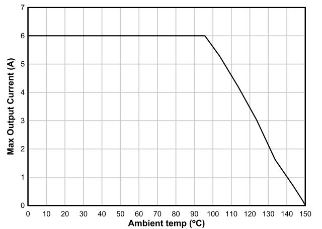
Figure 9-4. Maximum Output Current versus Ambient Temperature
