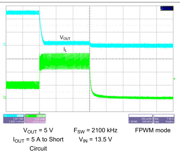
图 9-34. Short Circuit Protection
