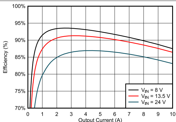
Figure 9-12. Efficiency
