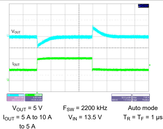
9-45. Load Transient
