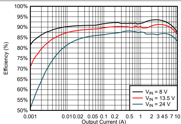
Figure 9-11. Efficiency
