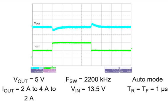
9-44. Load Transient
