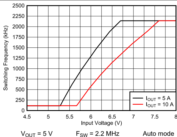
9-27. Frequency Dropout
