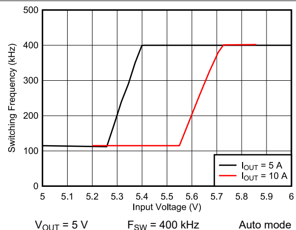
9-25. Frequency Dropout
