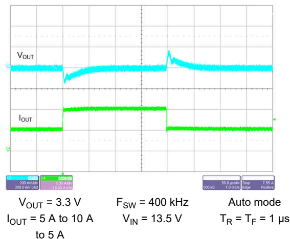
9-42. Load Transient
