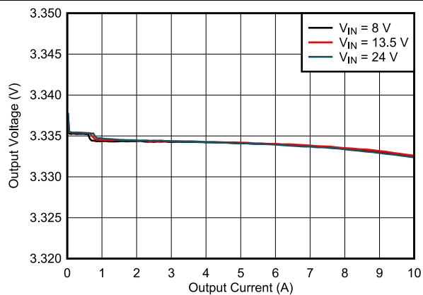
Figure 9-13. Load and Line Regulation
