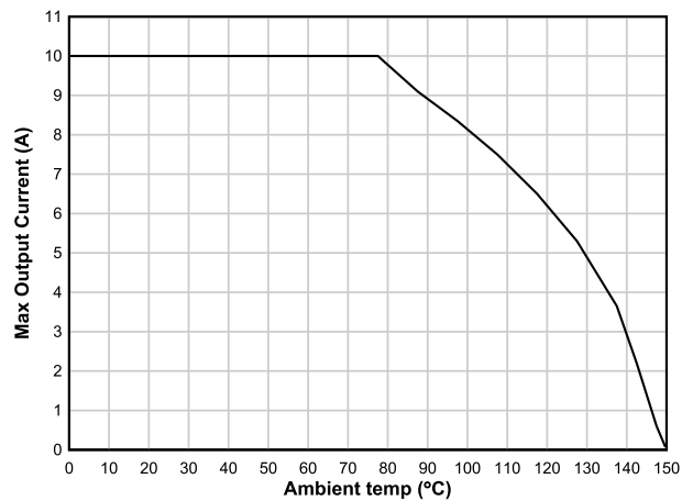
Figure 9-3. Maximum Output Current versus Ambient Temperature
