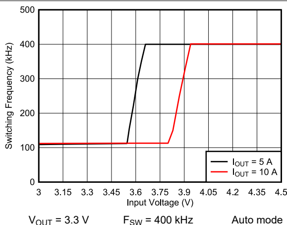
9-26. Frequency Dropout
