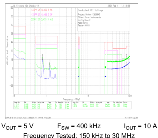
9-46. Conducted EMI versus CISPR25 Class 5 Limits (Green: Peak Signal, Blue: Average Signal)
