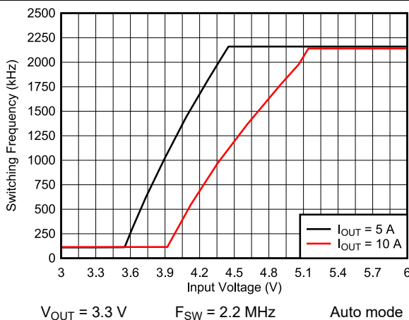
9-28. Frequency Dropout
