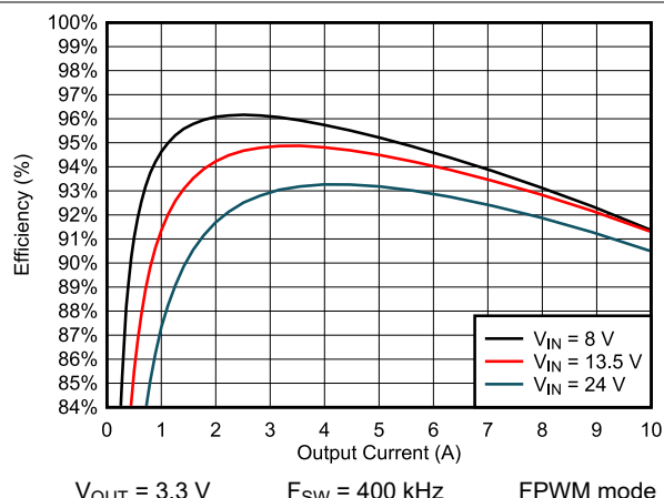
Figure 9-8. Efficiency
