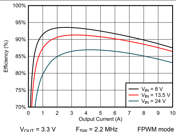
9-12. Efficiency
