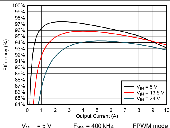
Figure 9-6. Efficiency
