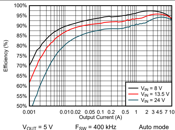
Figure 9-5. Efficiency
