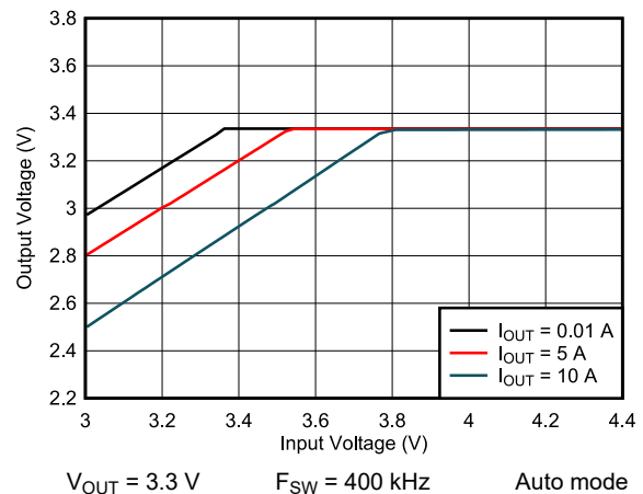
9-22. Dropout
