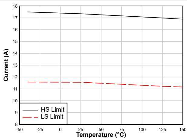
7-4. High-side and Low-side Current Limits
