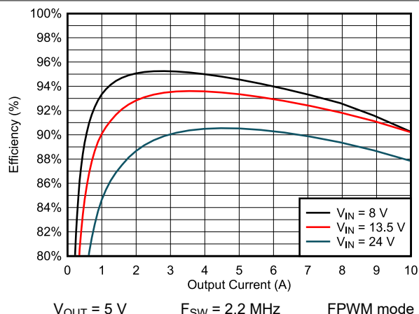
Figure 9-10. Efficiency
