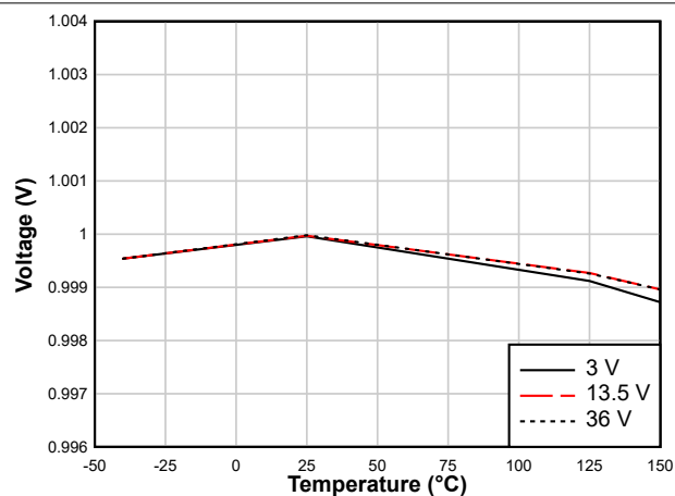
7-1. Feedback Voltage
