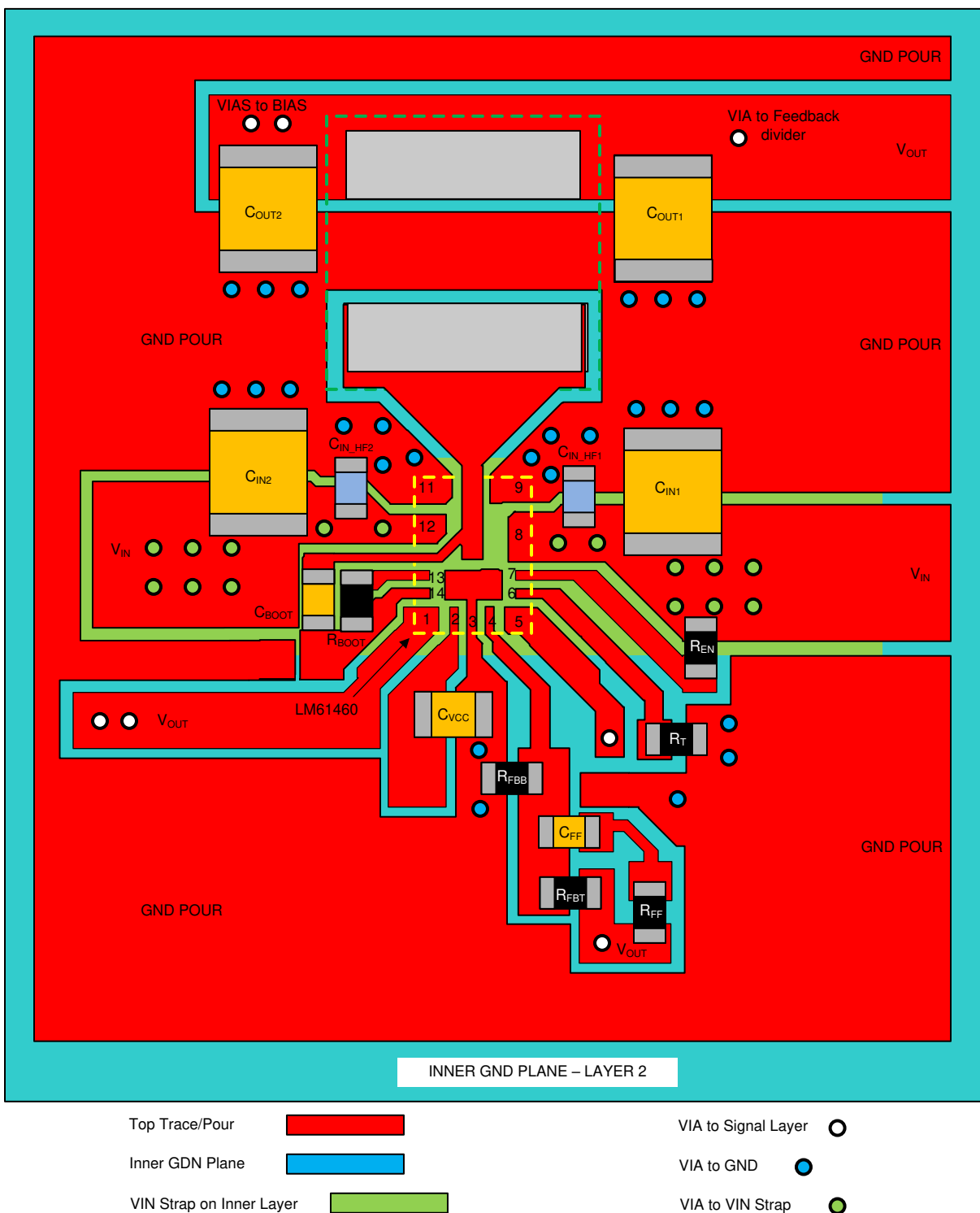
11-2. Layout Example
