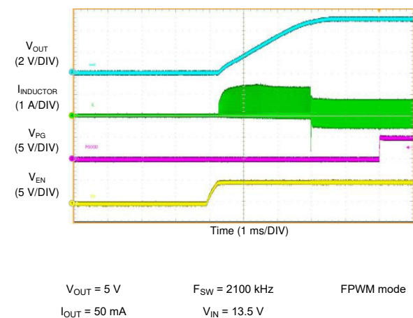
Figure 9-40. LM61460 Start-up with 50-mA
