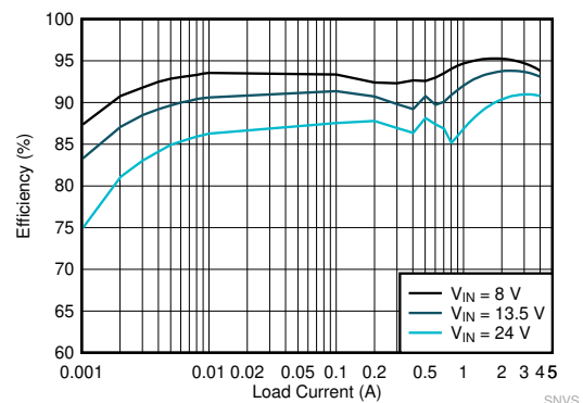
Efficiency V_{\text{OUT}} = 5 \text{ V} , f_{\text{SW}} = 2200 \text{ kHz}
