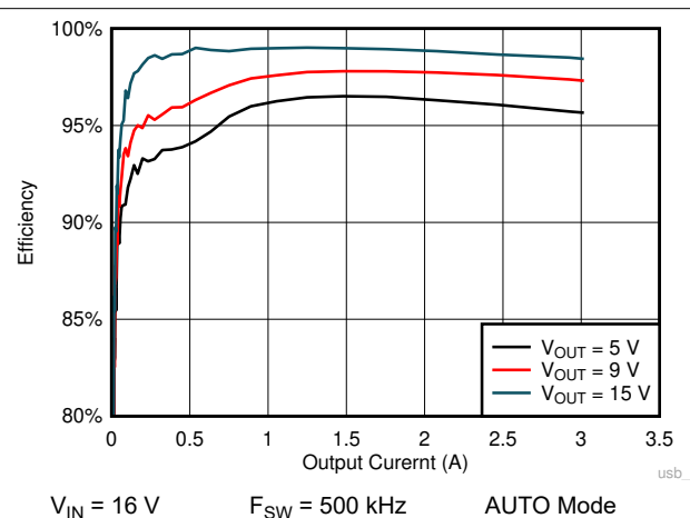
図 9-46. LM61460 Efficiency
