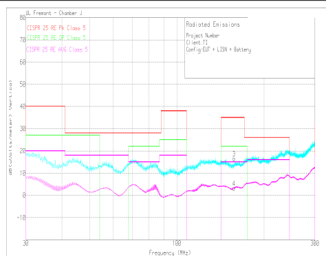
Figure 9-36. Radiated EMI Bicon Vertical versus CISPR25 Limits
