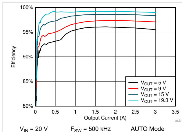
図 9-45. LM61460 Efficiency
