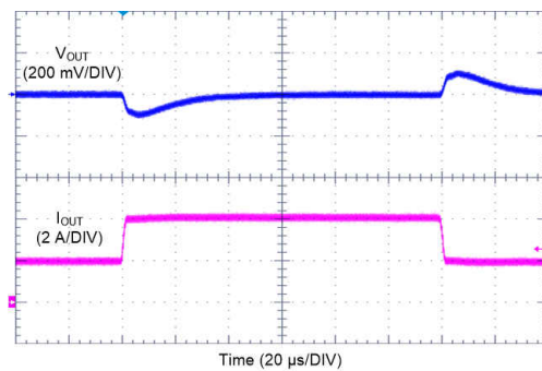
FIG 9-32. LM61440 Load Transient
