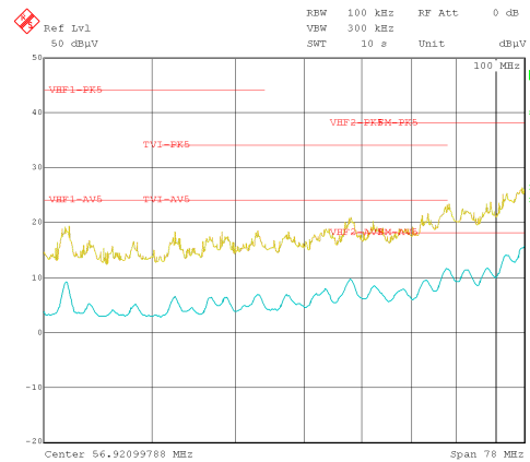
图 9-42. Conducted EMI versus CISPR25 Limits (Yellow: Peak Signal, Blue: Average Signal)
