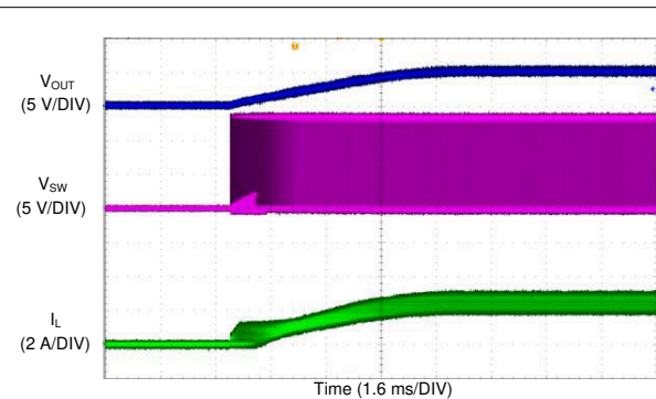
Figure 8-14. Short Circuit Recovery
