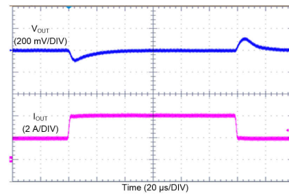
FIG 9-30. LM61440 Load Transient
