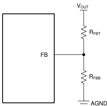
8-10. Setting Output Voltage of Adjustable Versions
