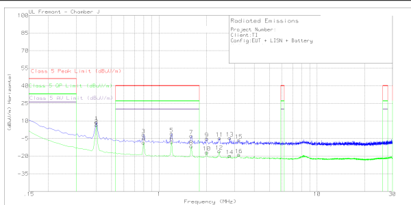
FIG 9-36. Radiated EMI Rod versus CISPR25 Limits
