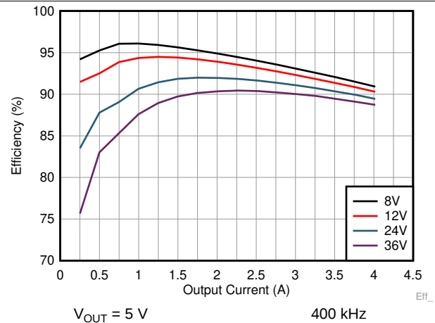
Figure 12. High-Load Efficiency
