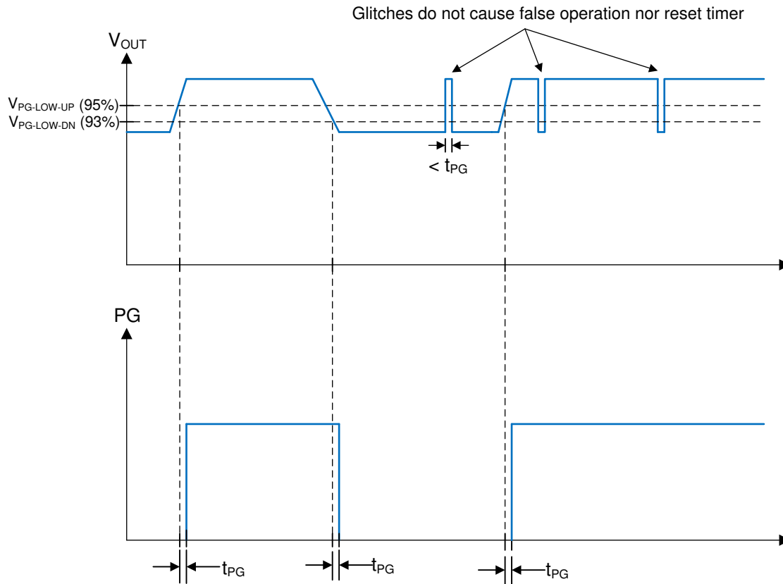
FIG 2. Power-Good-Timing Behavior
