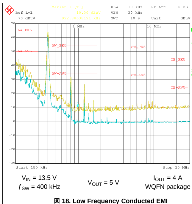
图 18. Low Frequency Conducted EMI
