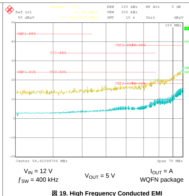
图 19. High Frequency Conducted EMI
